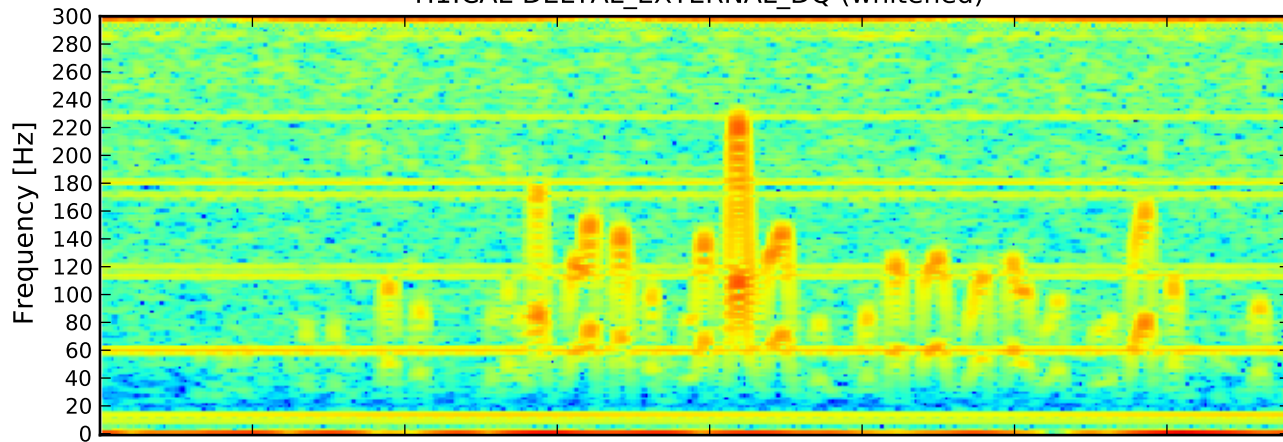
H1:CAL-DELTA_EXTERNAL_DQ (whitened)
