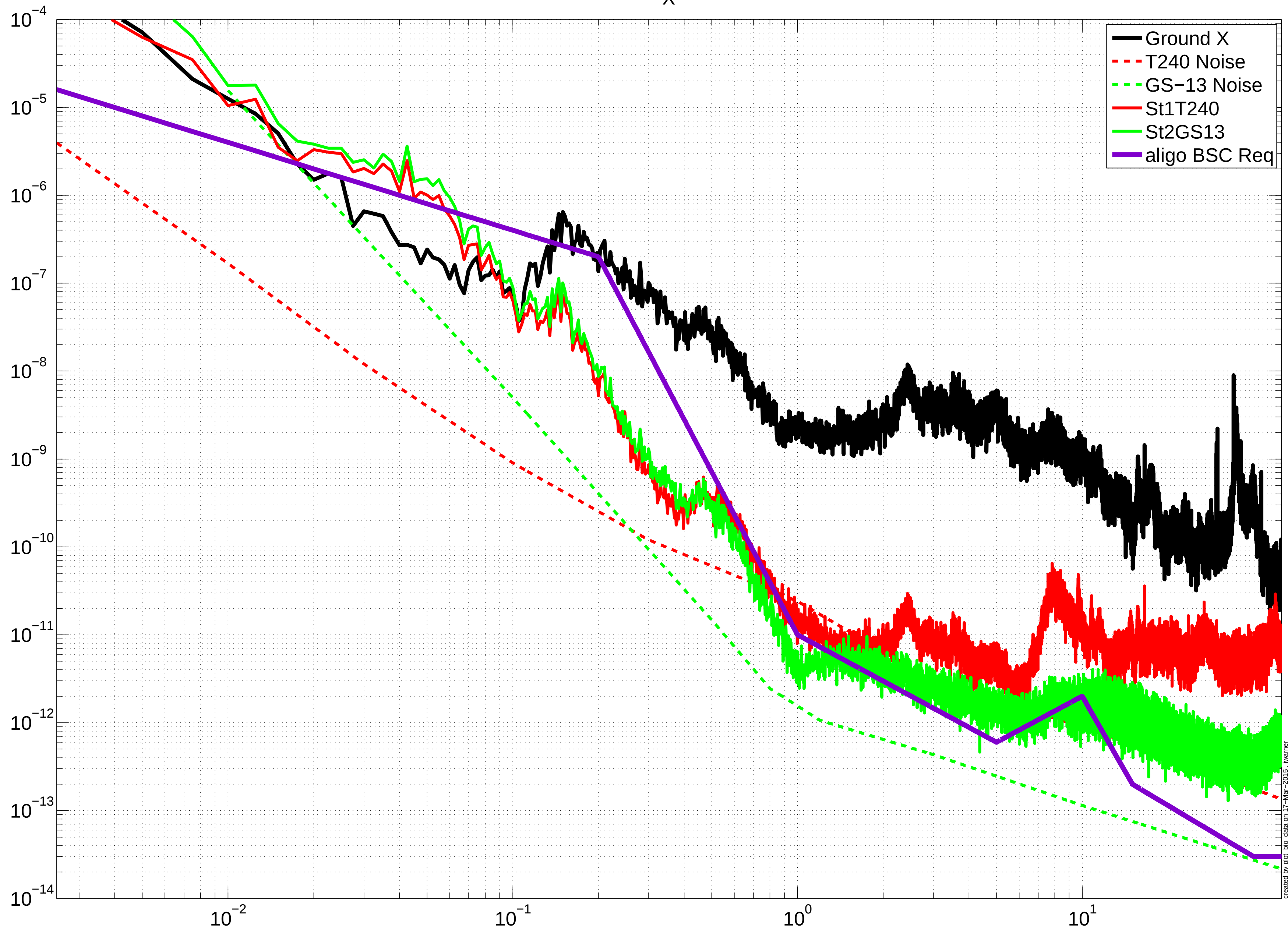
Final Performance, ETMX X
