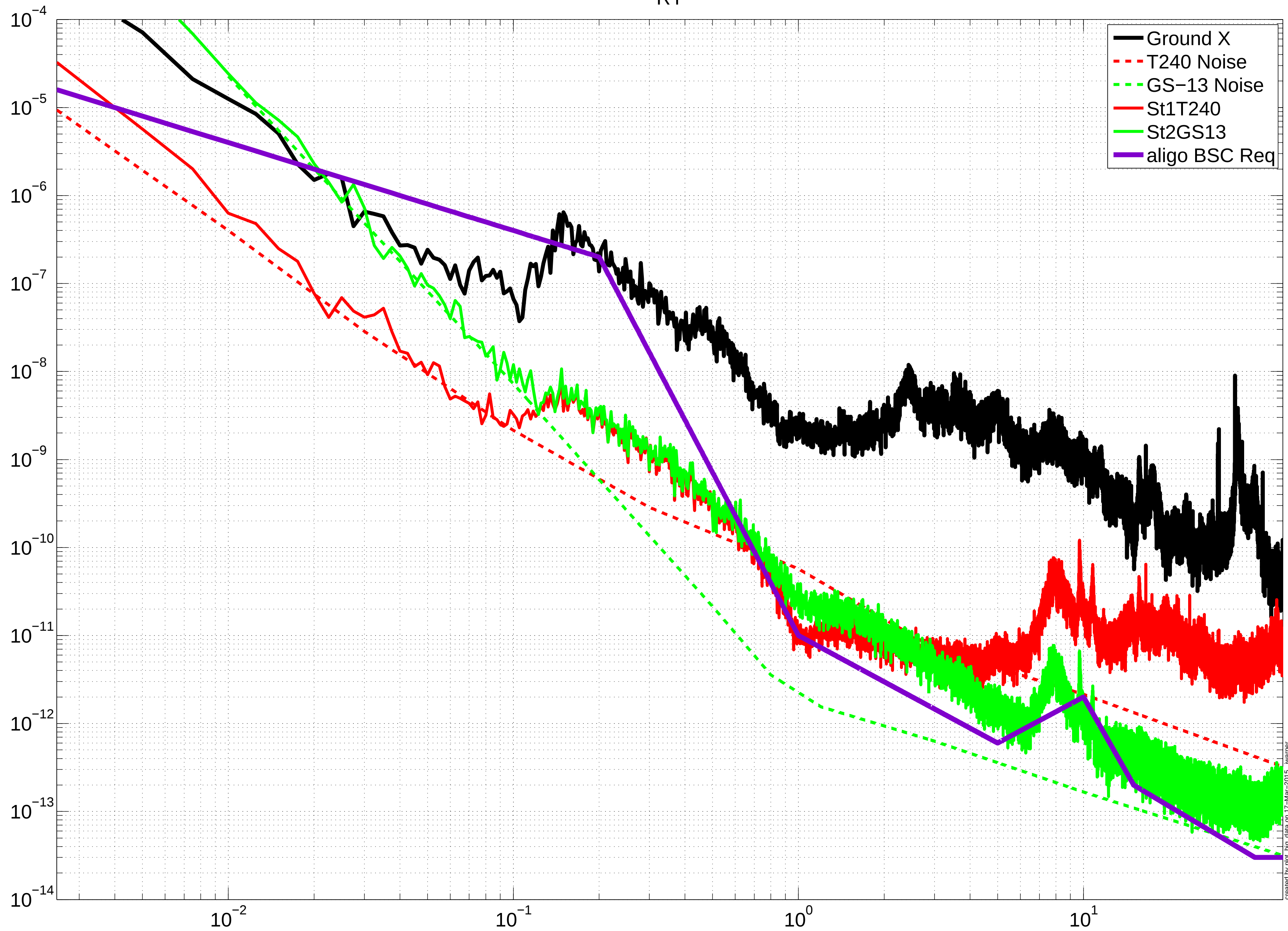
Final Performance, ETMX RY
