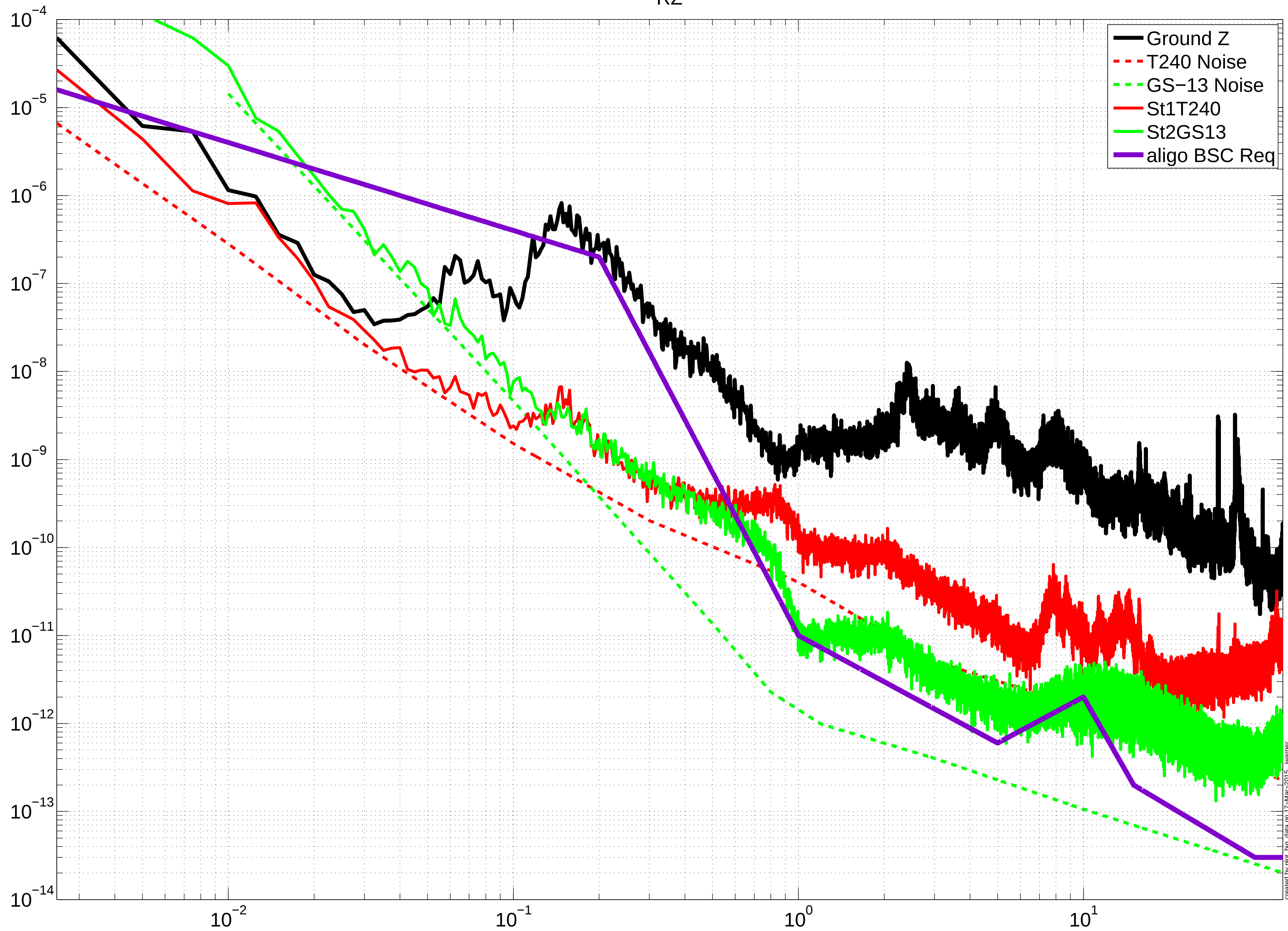
Final Performance, ETMX RZ
