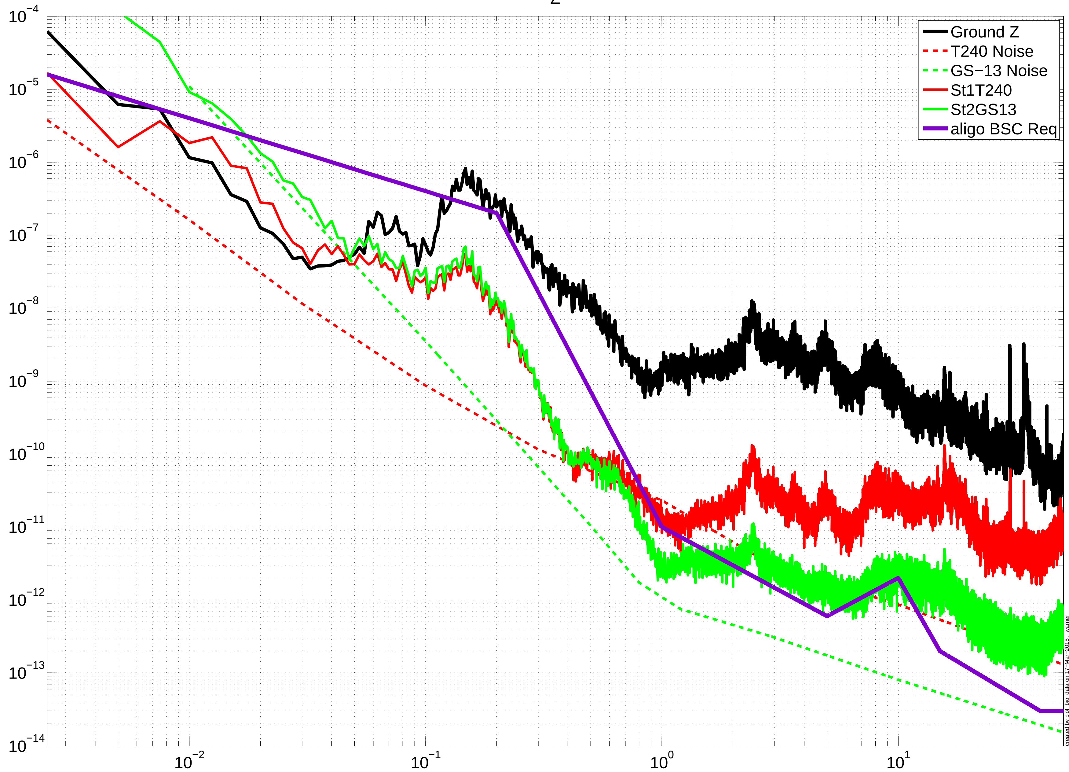
Final Performance, ETMX Z
