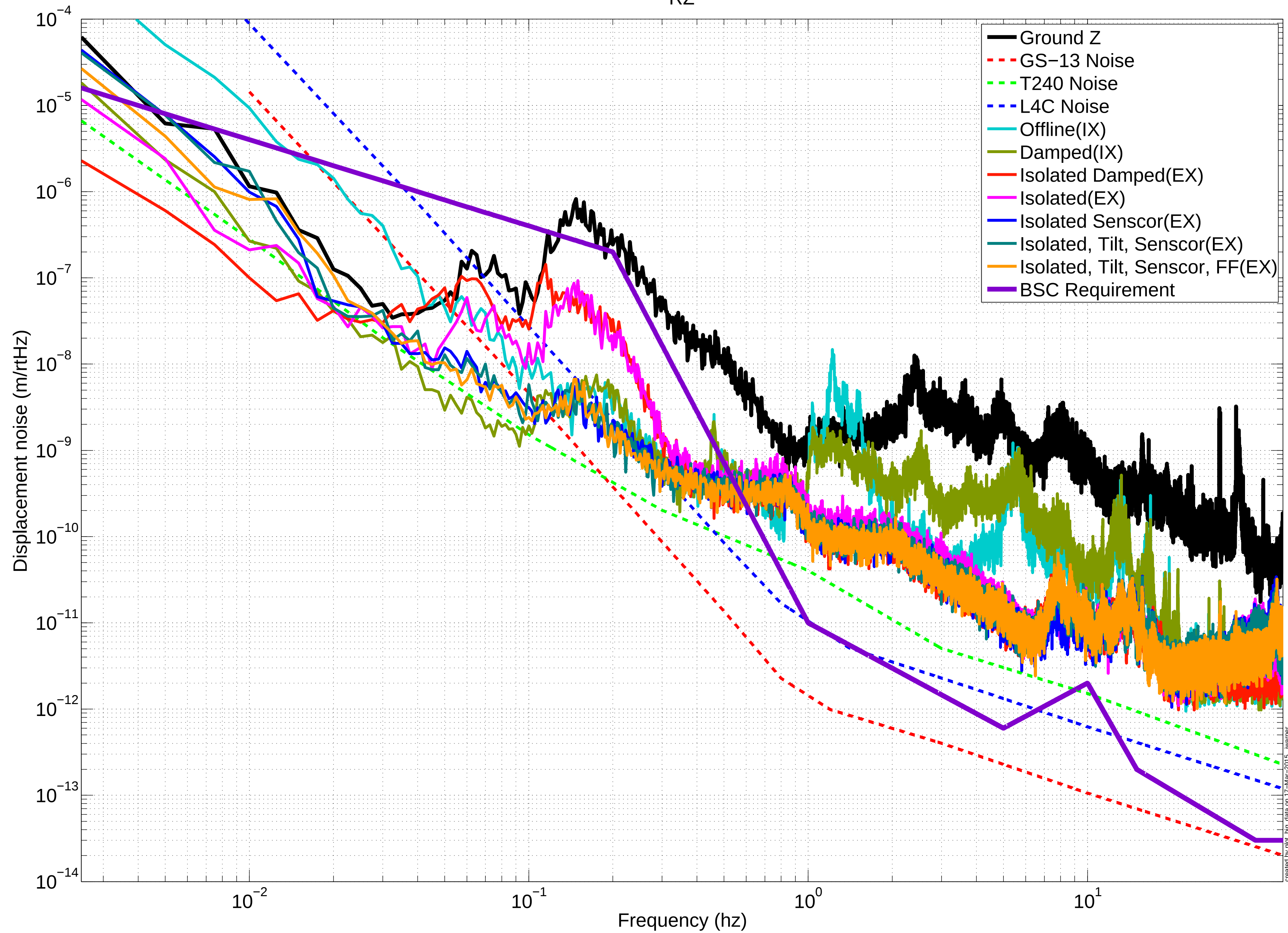
Control Contributions, St1 T240s RZ
