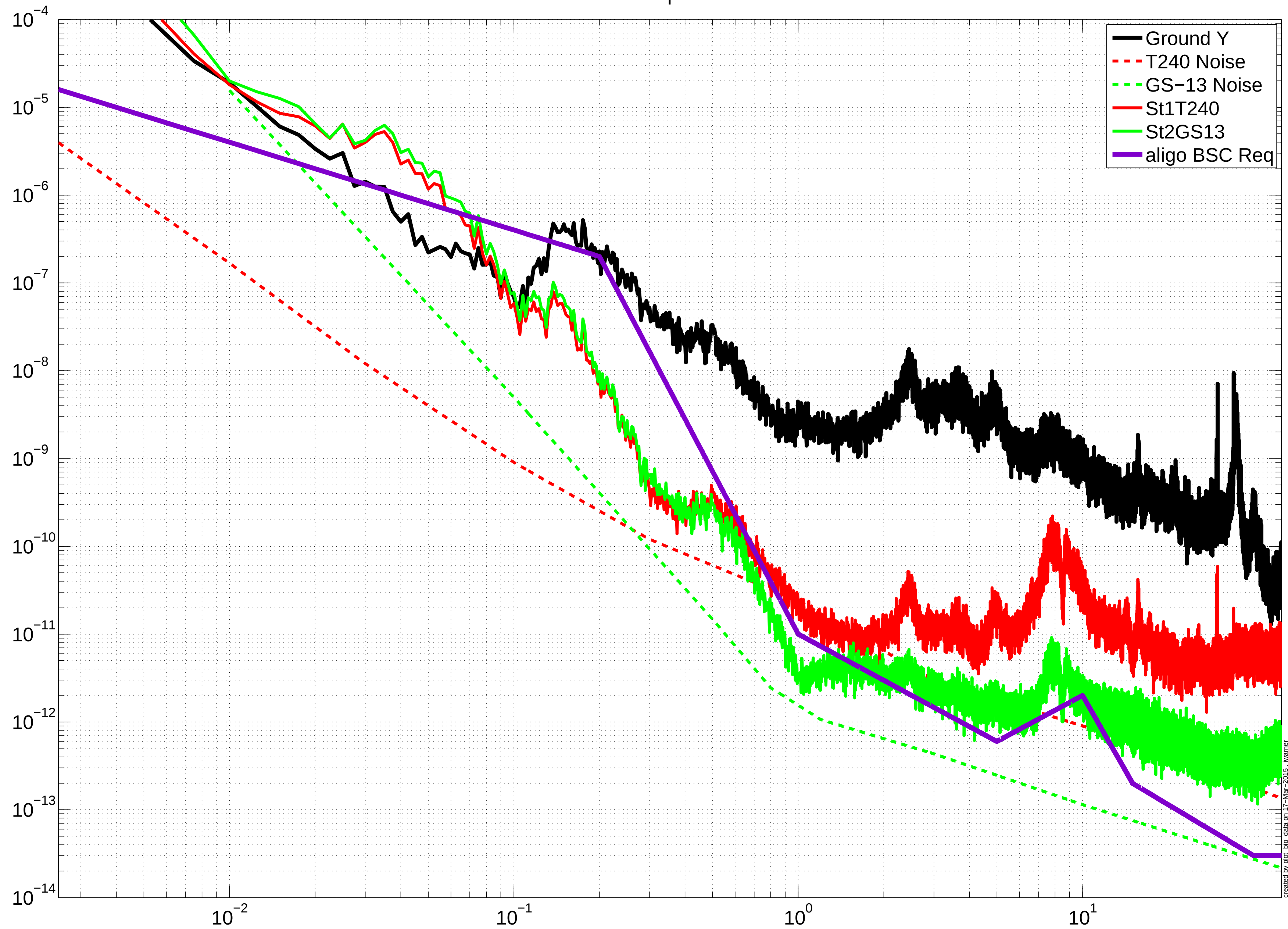
Final Performance, ETMX Y
