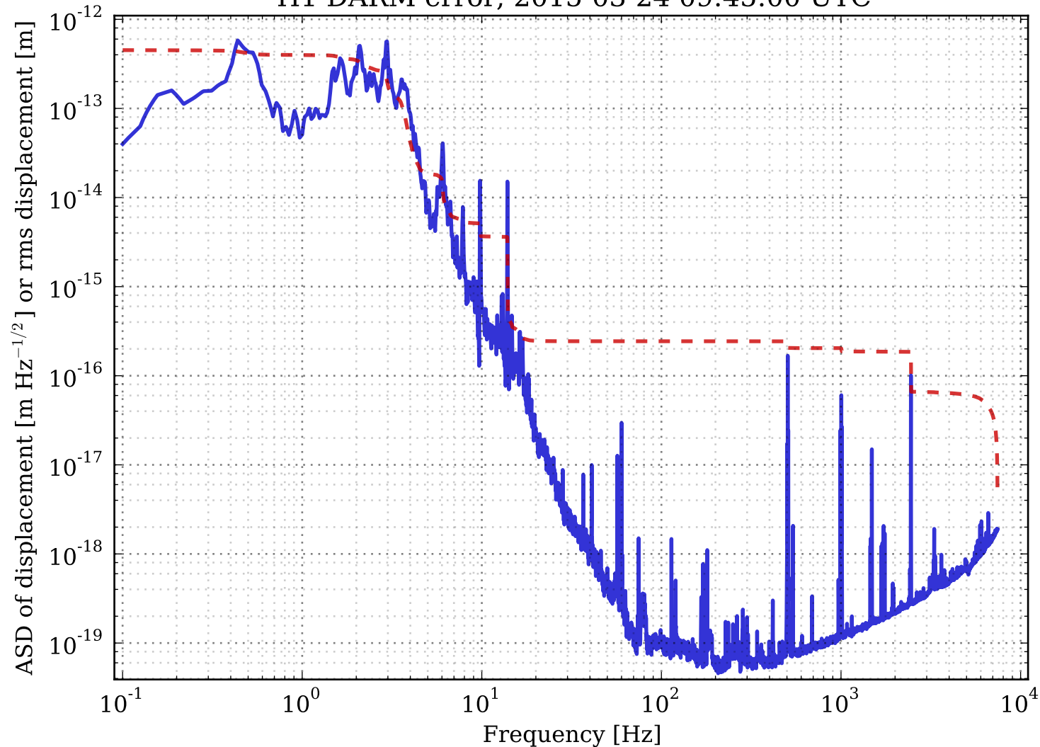
H1 DARM error, 2015-03-24 09:45:00 UTC
