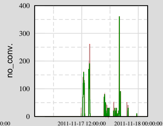
Ch 11: H0:PEM-LAB_DST1_5
