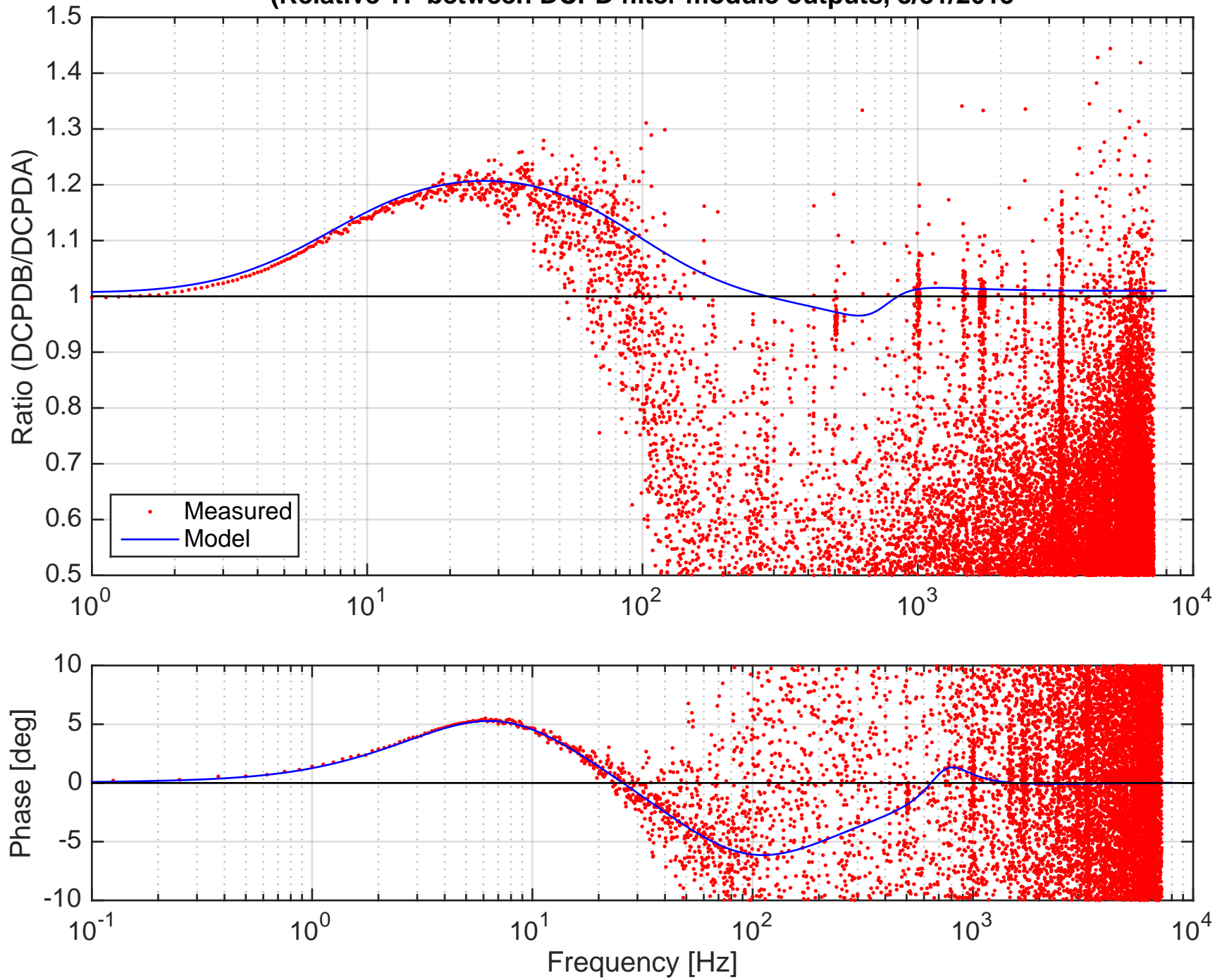
(Relative TF between DCPD filter module outputs, 3/31/2015)
