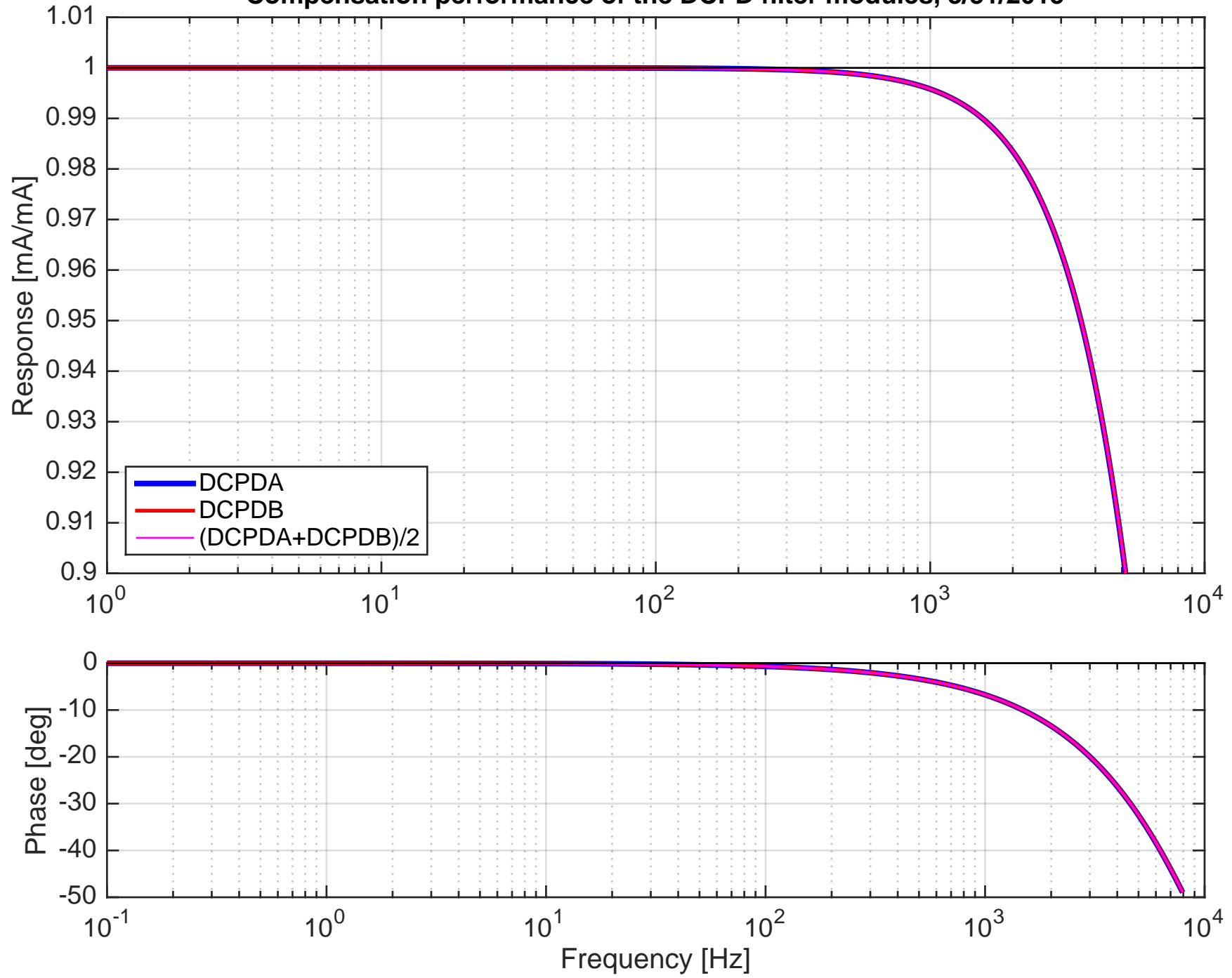
Compensation performance of the DCPD filter modules, 3/31/2015
