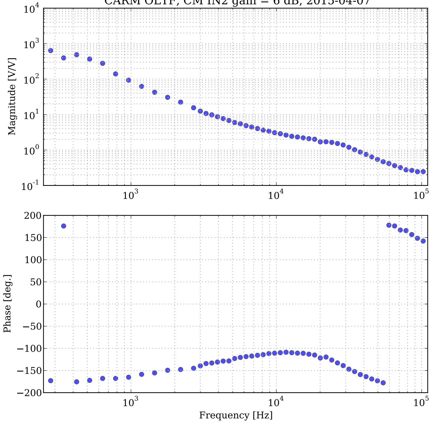
CARM OLTF, CM IN2 gain = 6 dB, 2015-04-07
