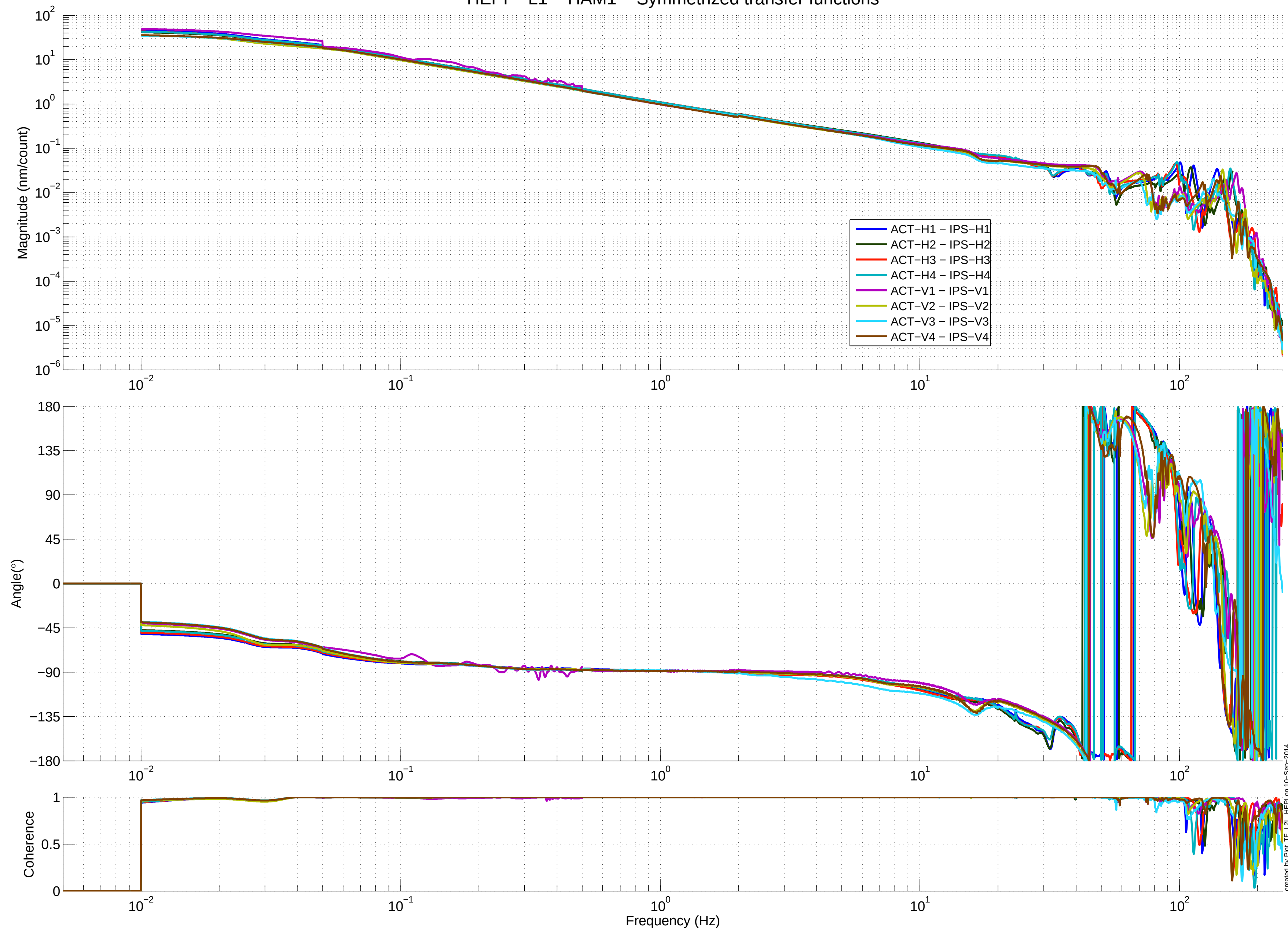
HEPI - L1 - HAM1 - Symmetrized transfer functions
