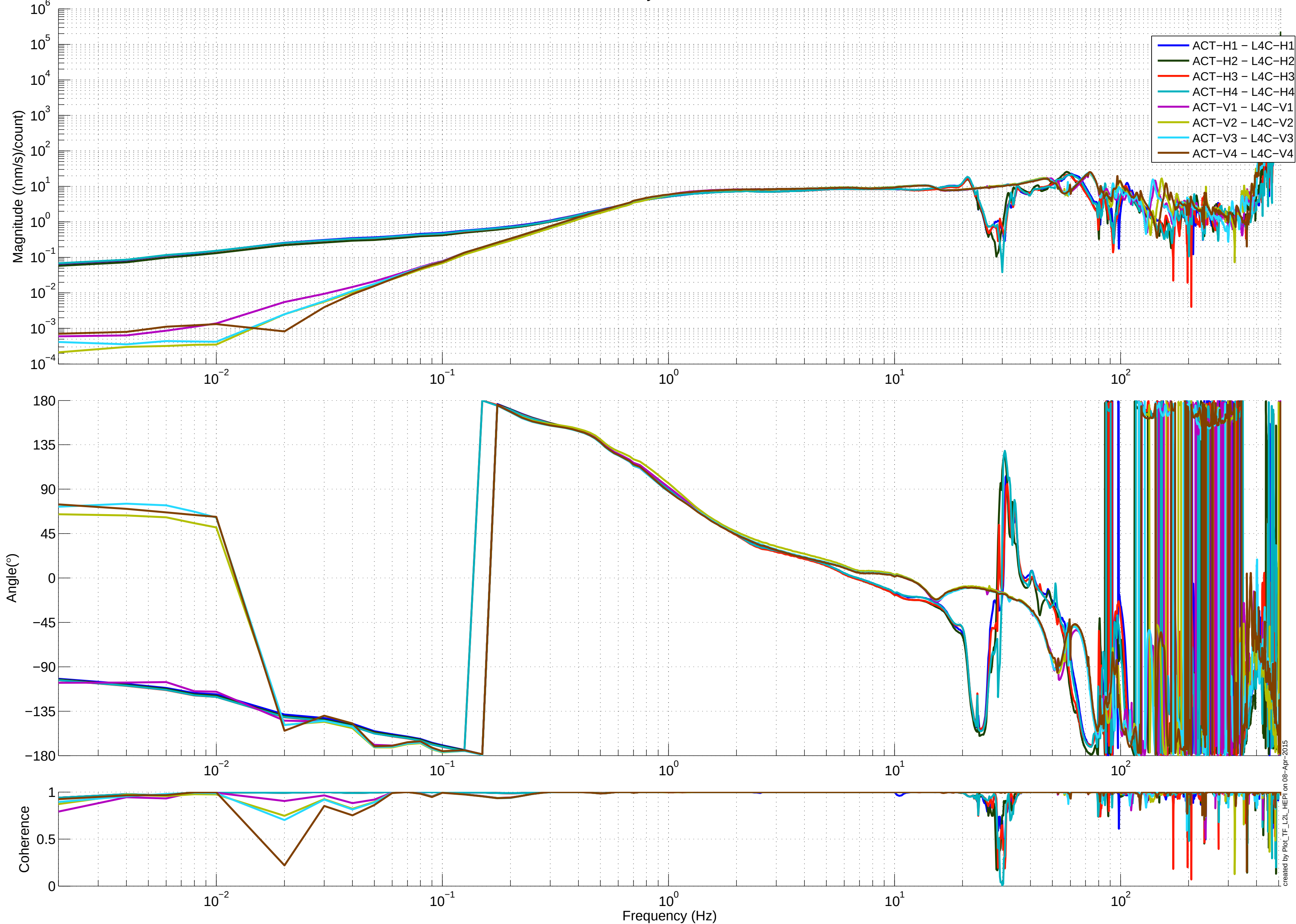
HEPI – H1 – HAM1 – Symmetrized transfer functions
