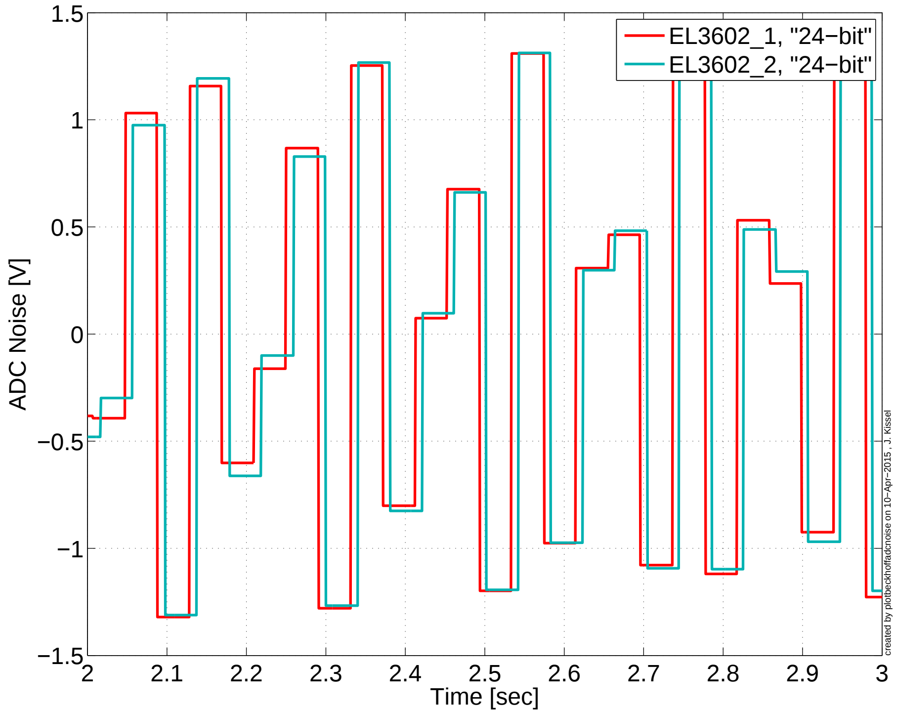
10 [Hz] Sine Wave, 1 [Vrms] Amplitude
