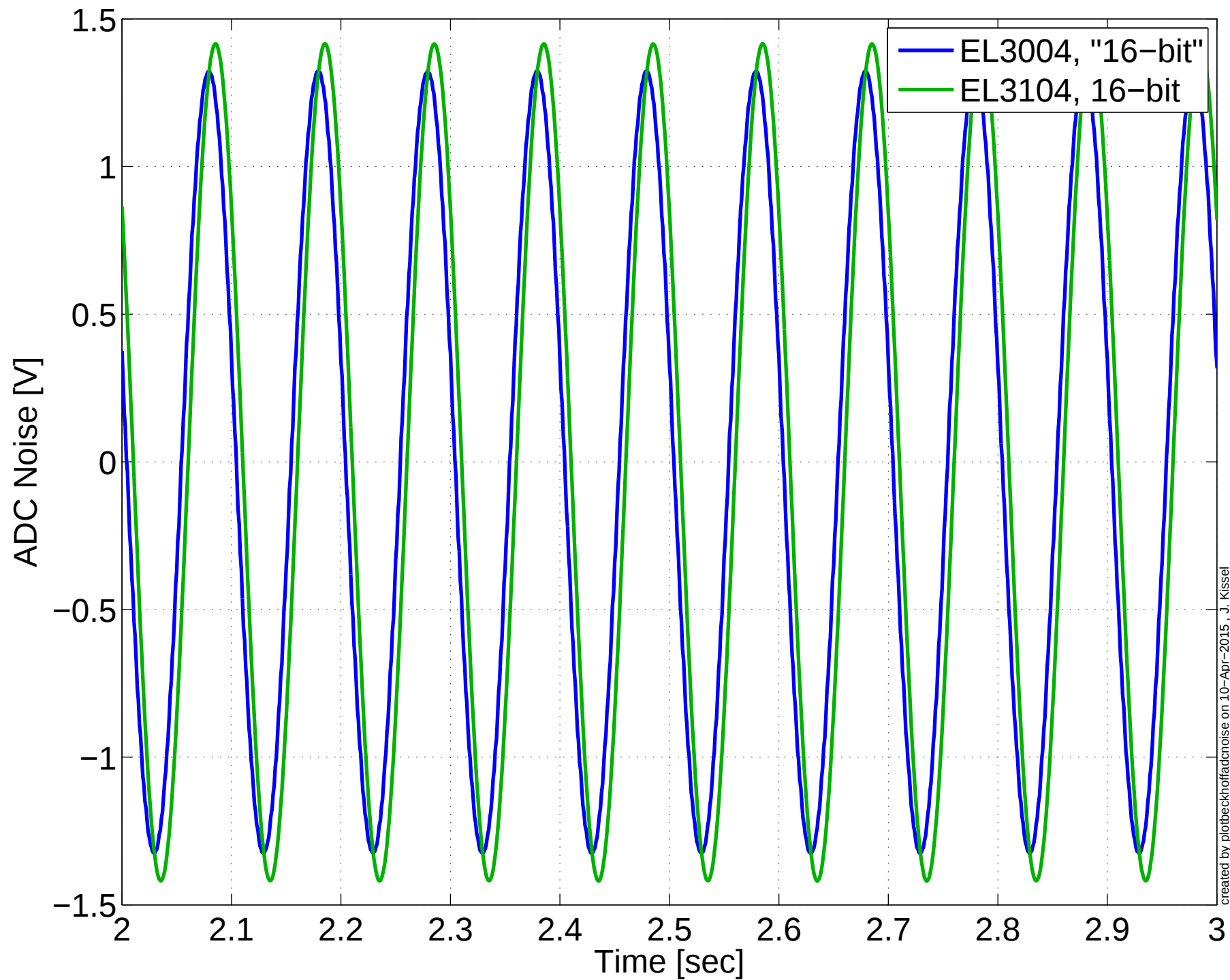
Input: 10 [Hz] Sine Wave, 1 [Vrms] Amplitude
