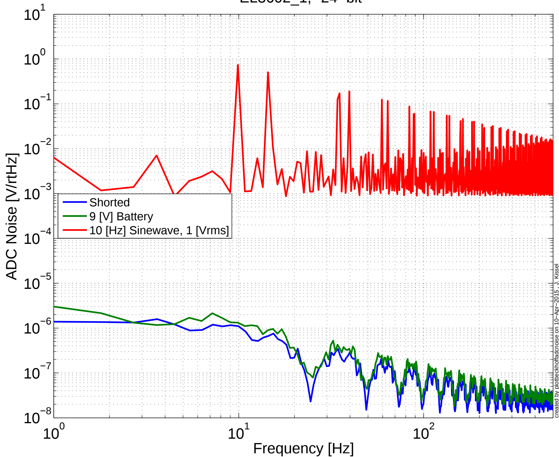
EL3602_1, "24-bit"
