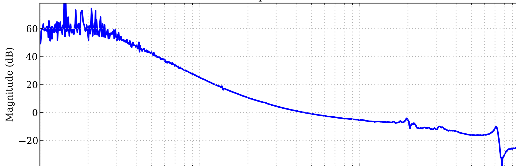
IMC OLTF - Apr 11 2015 - 19:51:45
