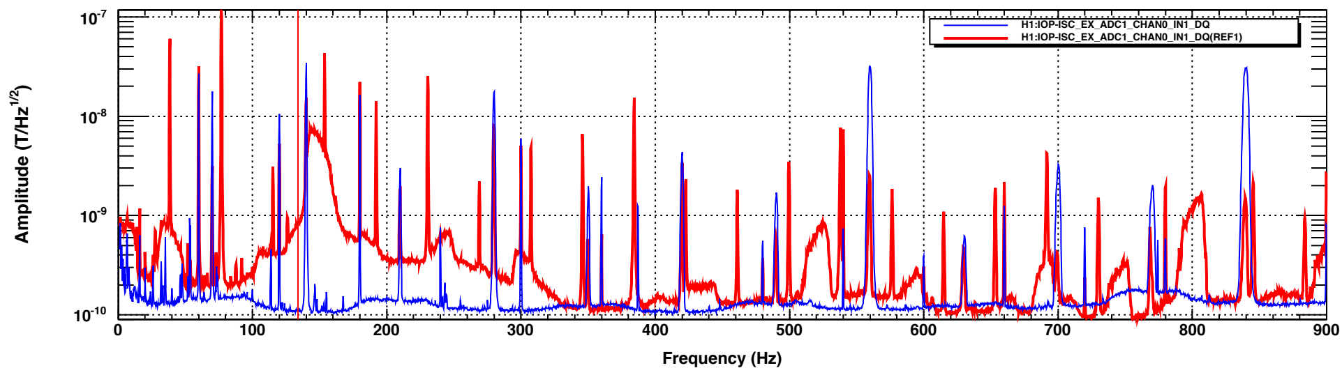
Magnetic field, magnetometer on power supply, RED: original, BLUE: new
