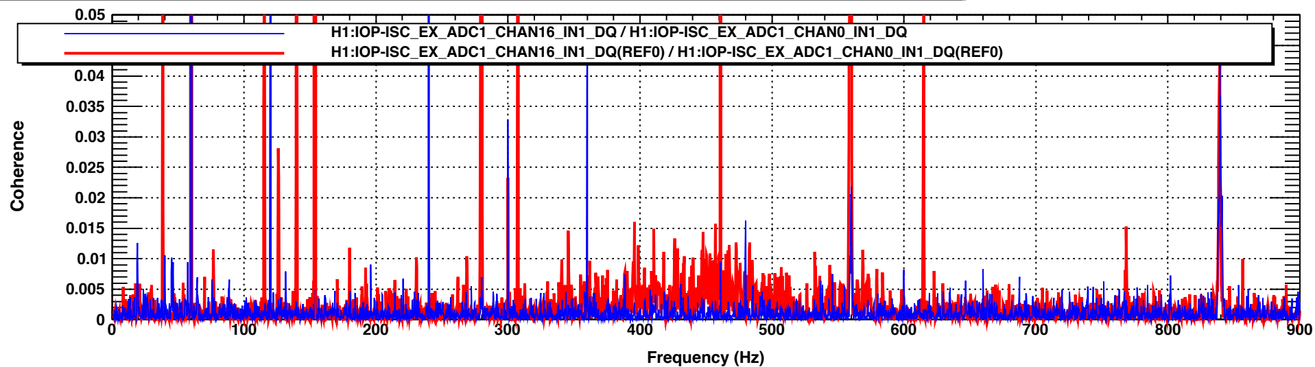
Coherence between magnetometer channel and channel terminated at AA chasis, RED original supply, BLUE: new, high only at 60 Hz harmonics
