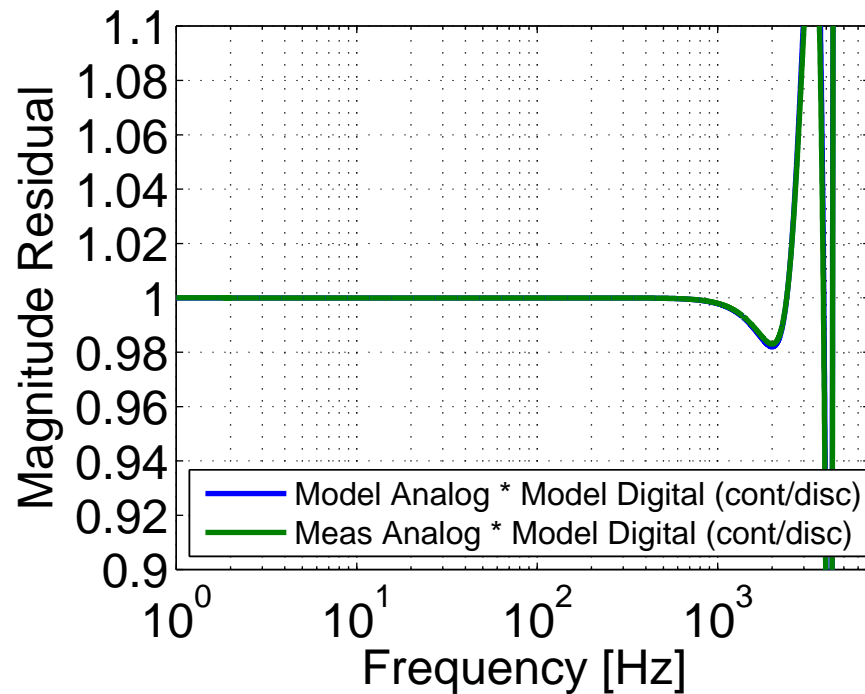
Continuous / Discrete
