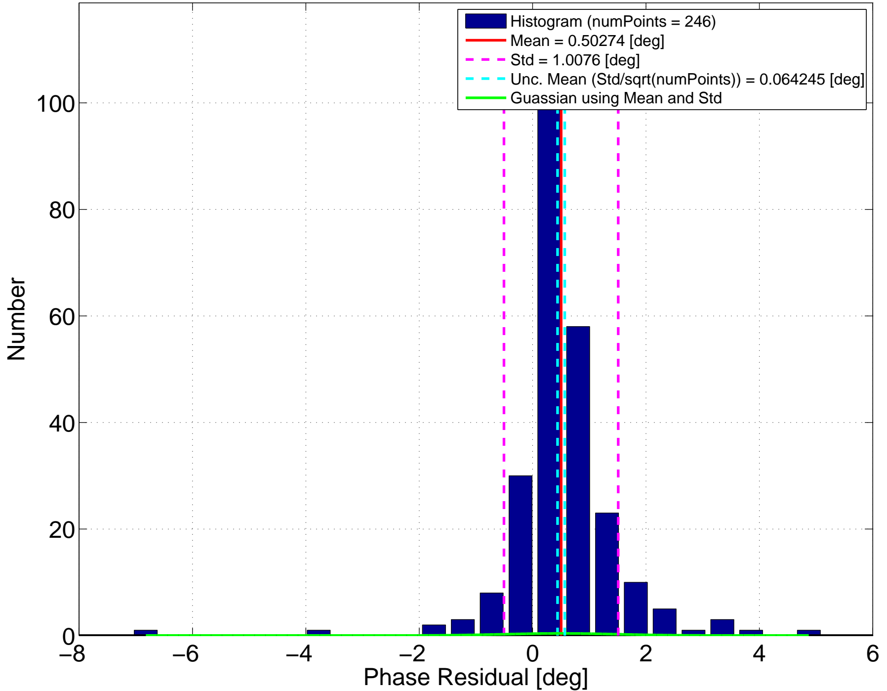
H1 DARM Open Loop Gain TF Histogram 2015-05-02 Phase Residuals (numMeas = 8)
