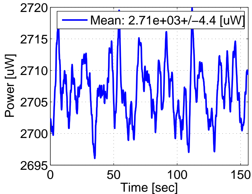
Power @ IM4 Trans
