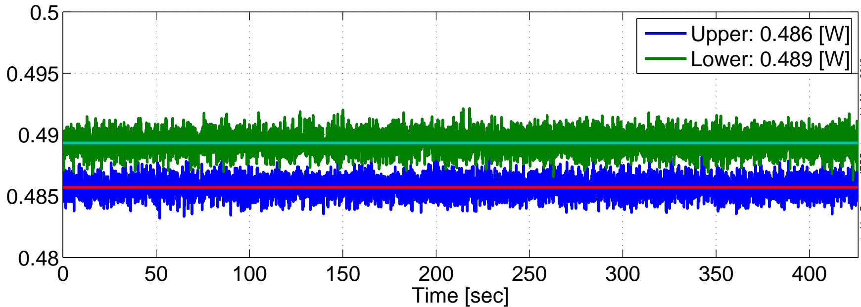
H1 DARM OLGTF, May 07 2015 07:08:12 UTC TCS ETMX Ring Heater Power
