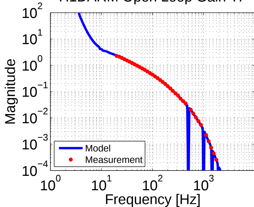
H1DARM Open Loop Gain TF
