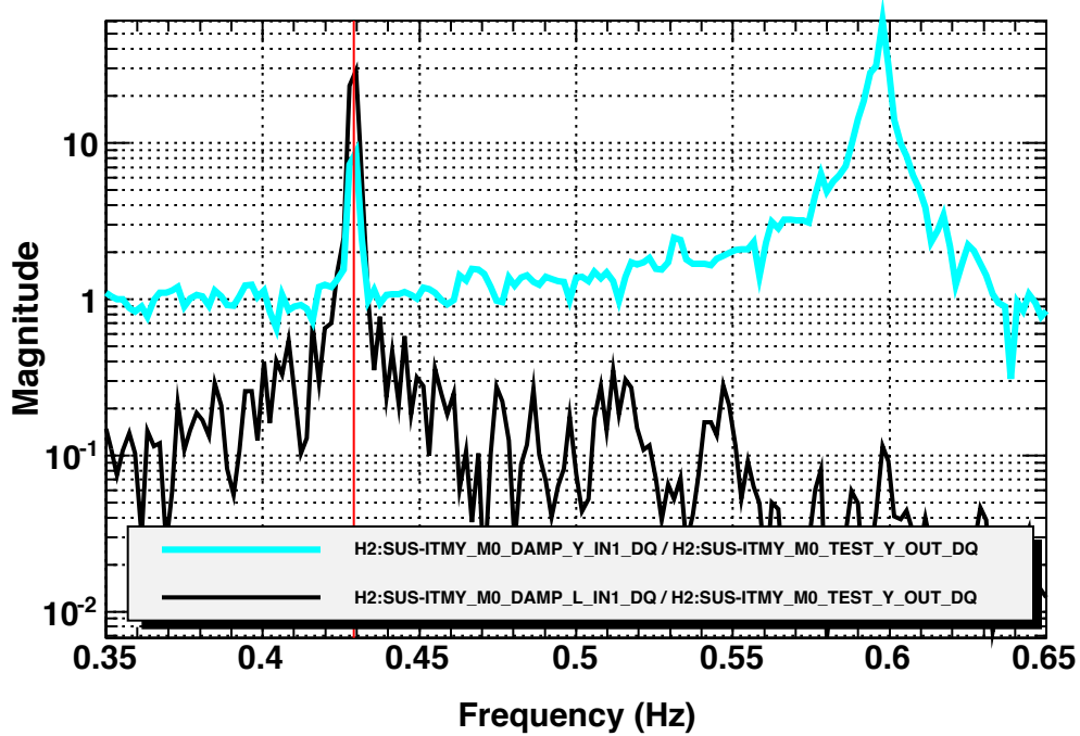
Transfer function
