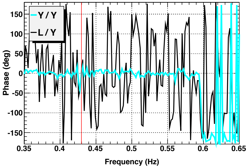
Transfer function
