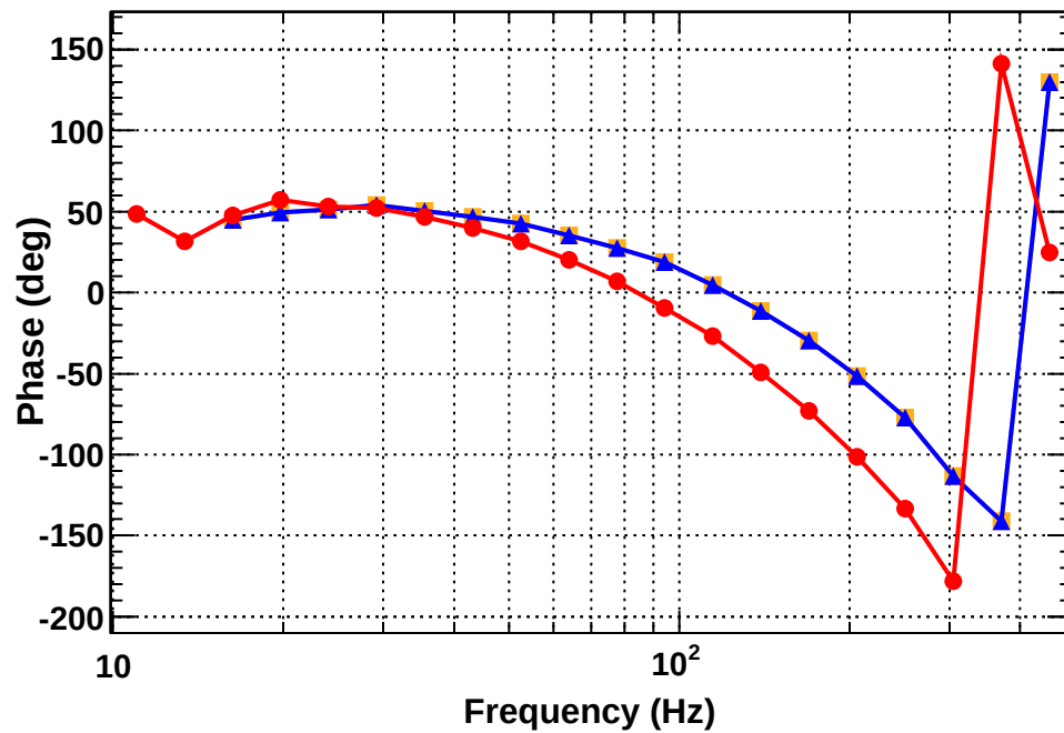
Transfer function
