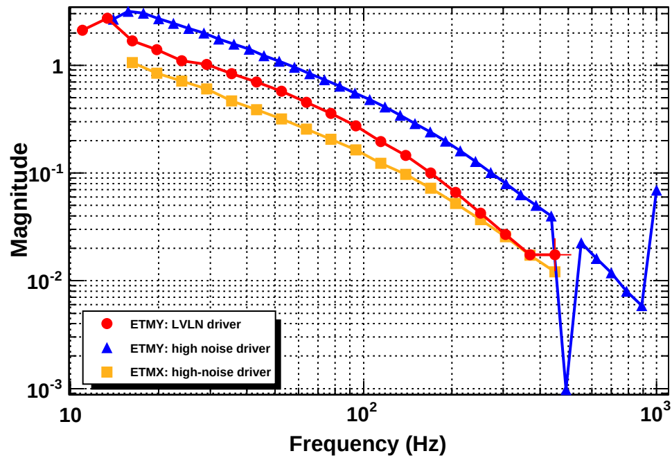
Transfer function
