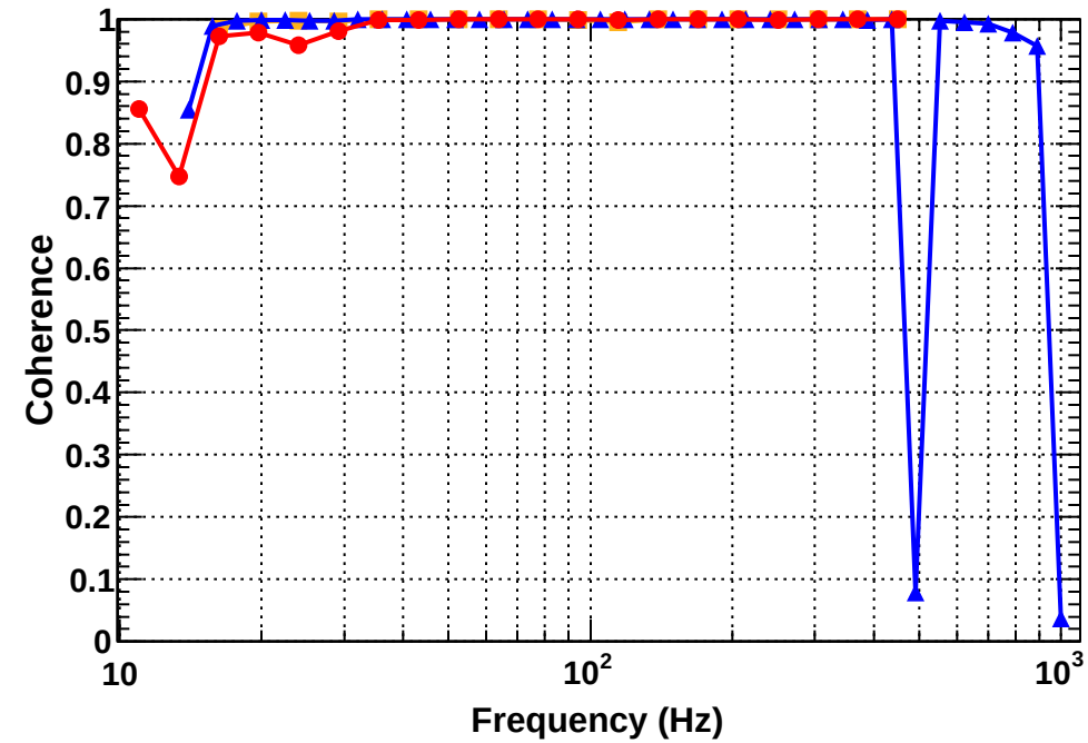
Coherence function
