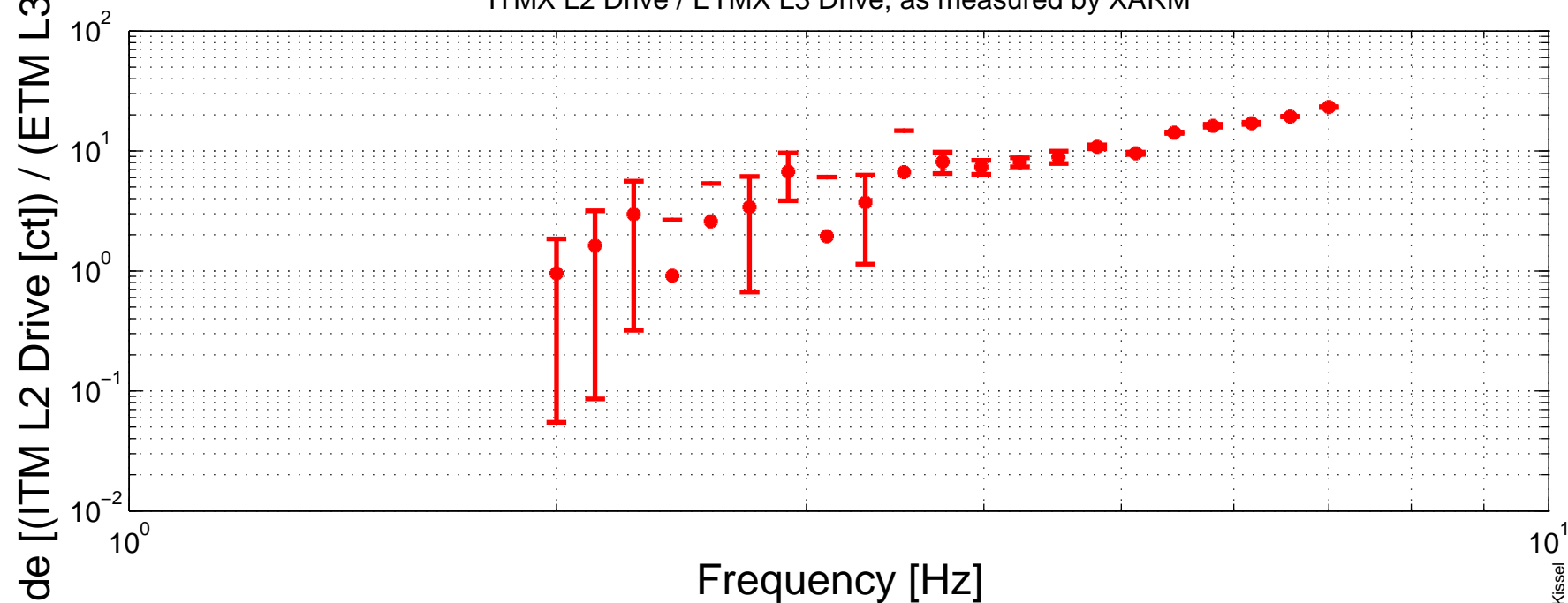
2015-05-28, H1 Free-Swinging MICH Meas ITMX L2 Drive / ETMX L3 Drive, as measured by XARM
