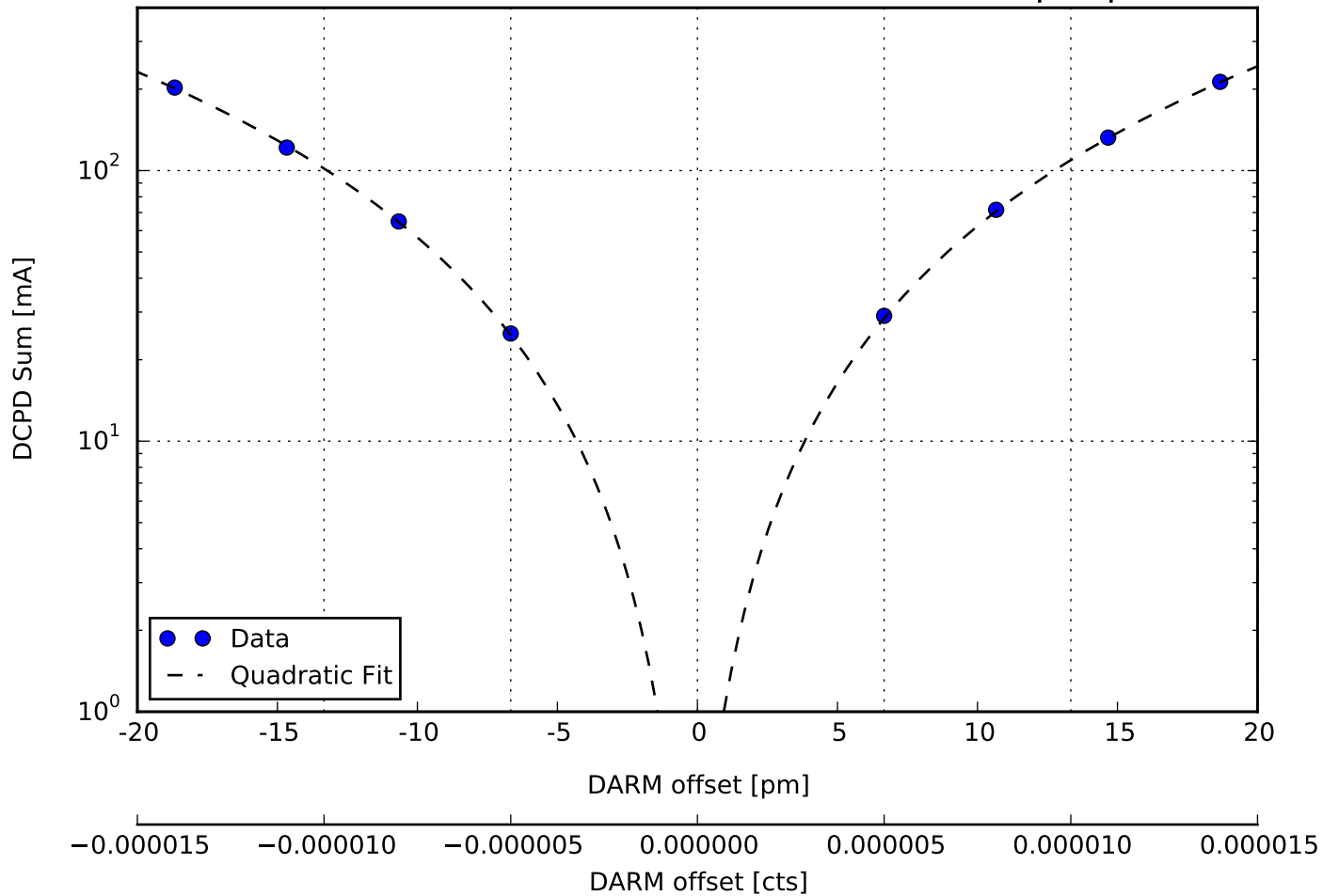
DCPD Sum vs DARM offset - scaled for 125W input power
