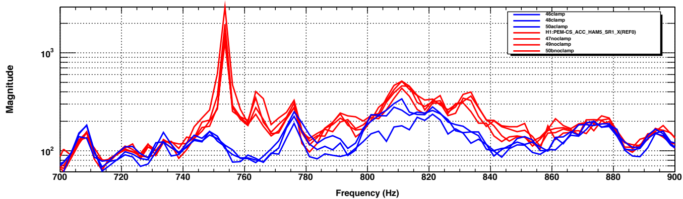
Accel. near suspension, taps on ISI suspension wire loc. 3, BLUE: damping clamp on wire, RED: no clamp, all blue traces in front of red
