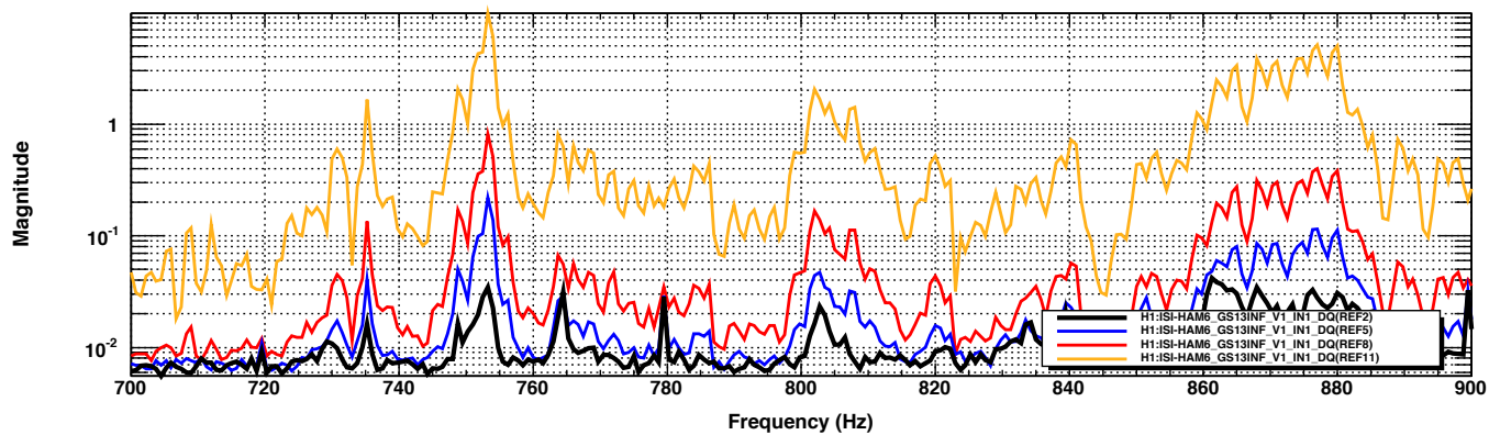
HAM6 GS13s, shaker on HAM6 blue beam, 700-900 Hz injection, BLACK: no shaking
