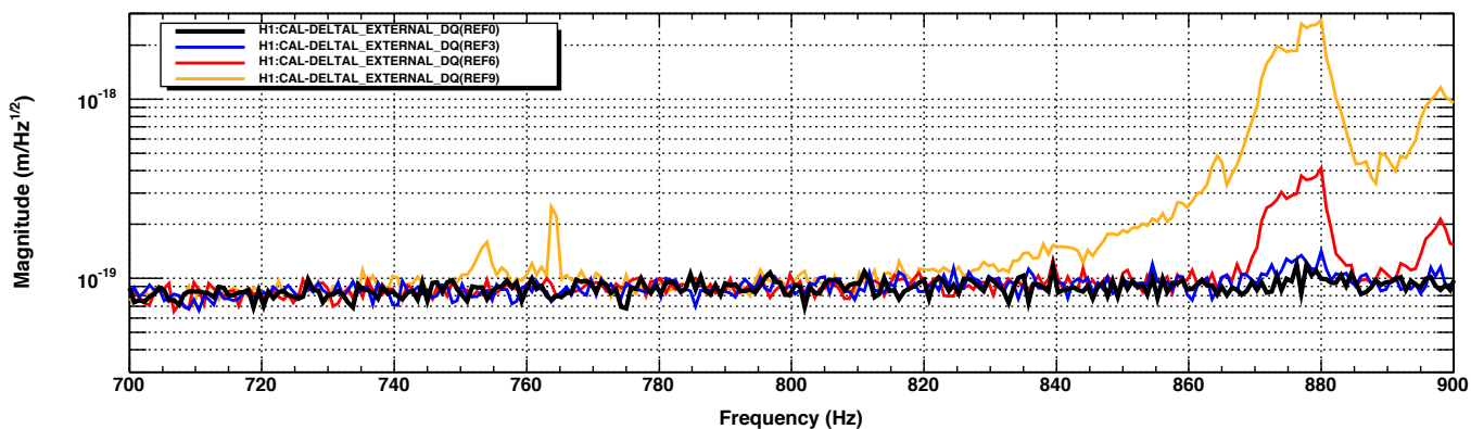
DARM during HAM6 shaking, BLACK: no shaking
