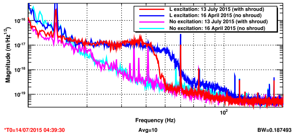
aLIGO DARM: OMC Scattering L
