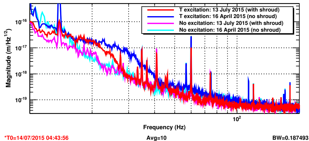
aLIGO DARM: OMC Scattering T
