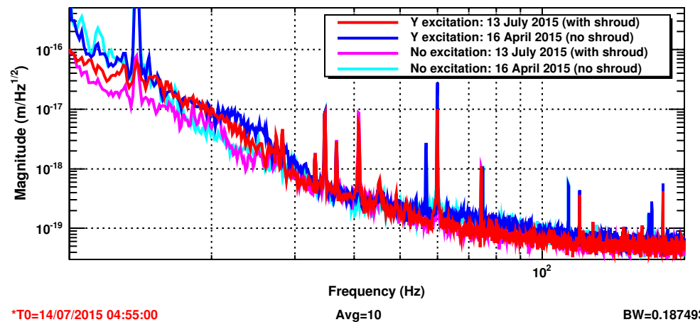
aLIGO DARM: OMC Scattering Y
