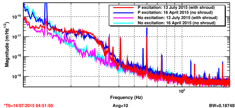
aLIGO DARM: OMC Scattering P
