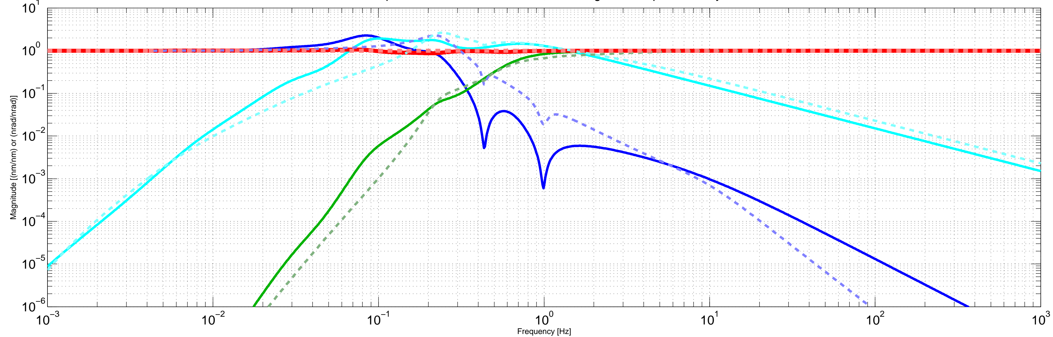
H1ISIETMY ST1 Quite and Windy RY Blend Filters Displacement LP vs Inertial HP, As Designed Complementarity
