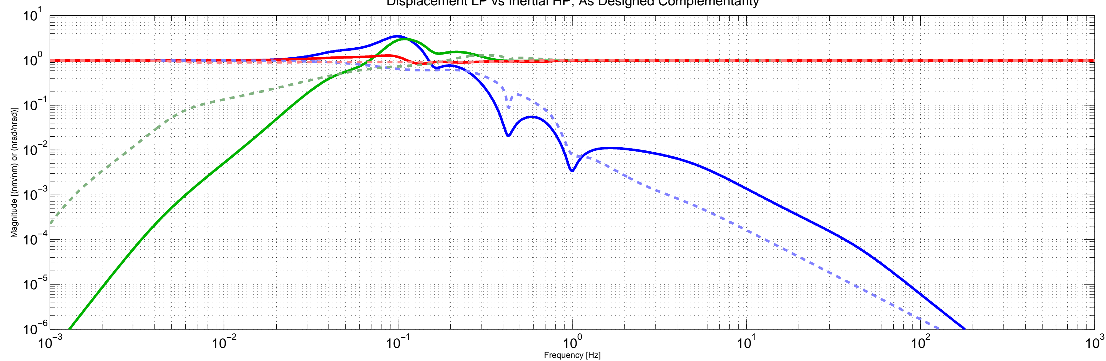
H1ISIETMY ST1 Quite and Windy RY Blend Filters Displacement LP vs Inertial HP, As Designed Complementarity
