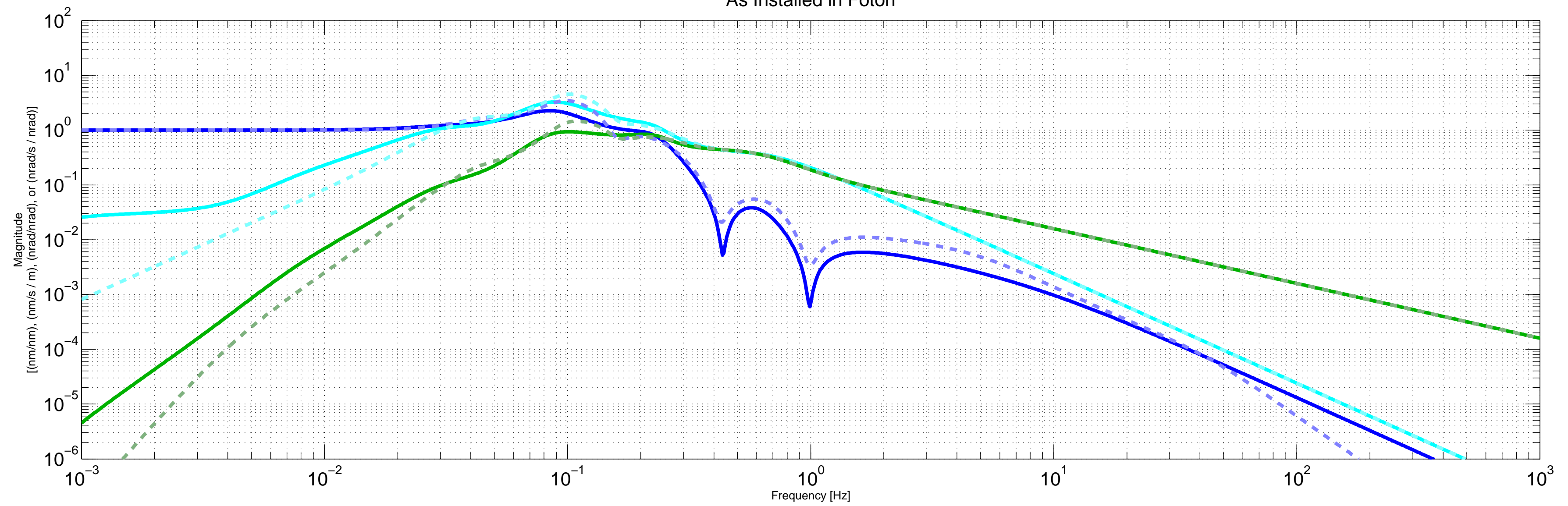
H1ISIETMY ST1 X Quite and Windy Blend Filters As Installed in Foton
