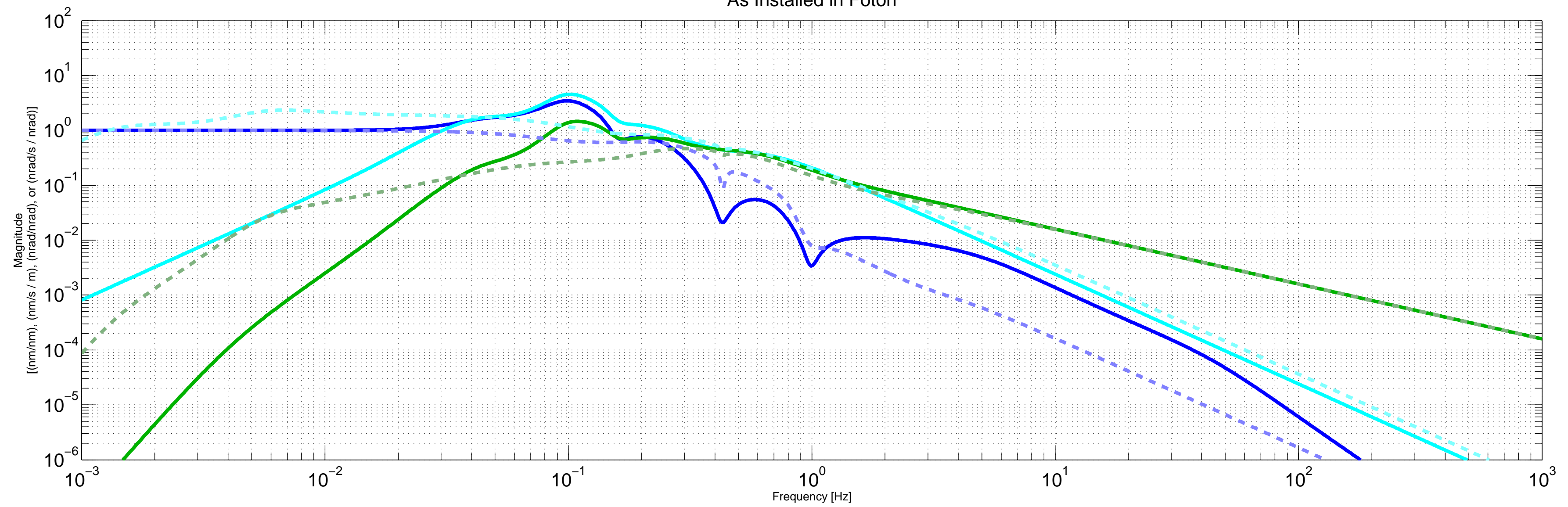
H1ISIETMY ST1 RY Quite and Windy RY Blend Filters As Installed in Foton
