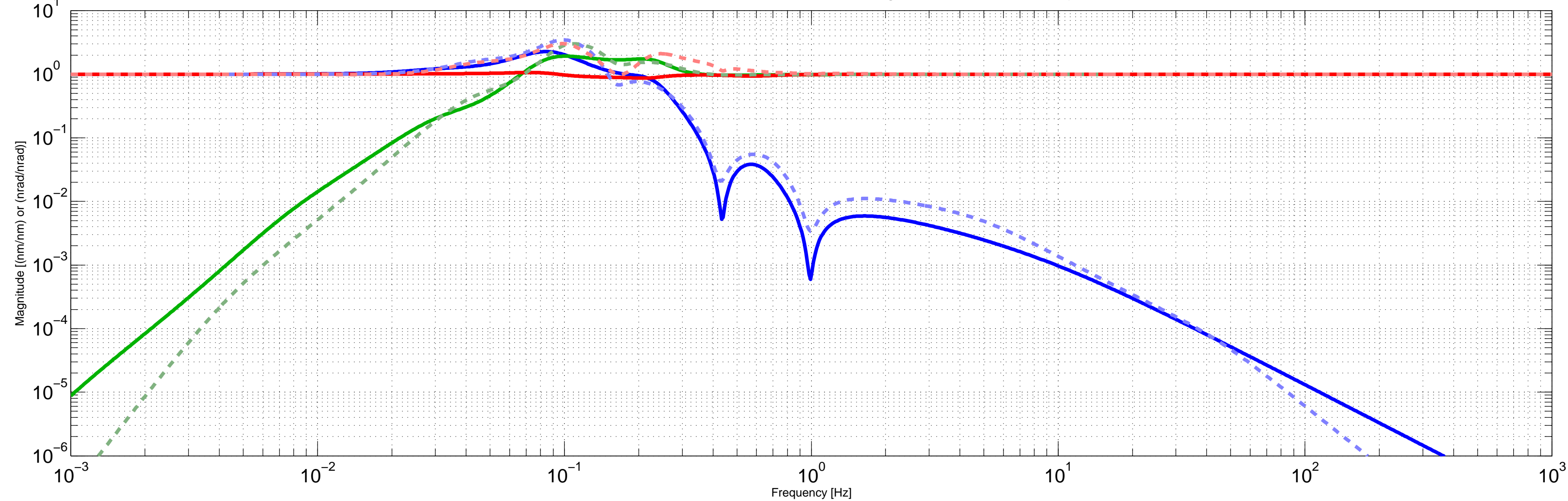
H1ISIETMY ST1 X Quite and Windy Blend Filters Displacement LP vs Inertial HP, As Designed Complementarity
