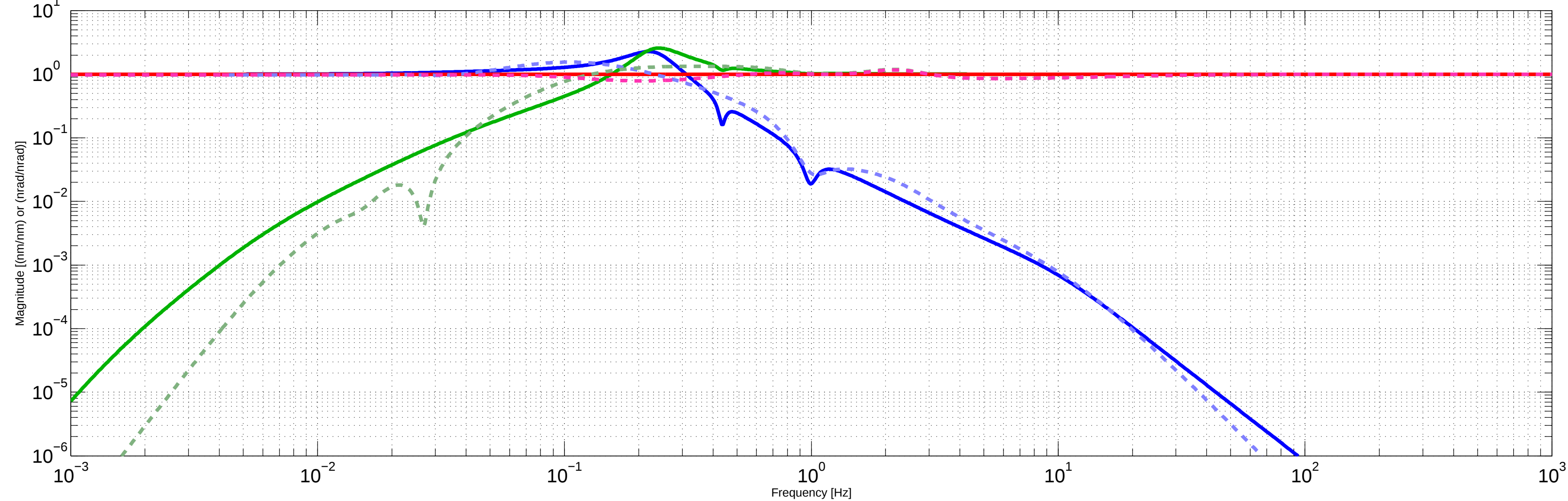
H1ISIETMX ST1 RY Quite and rdr Blend Filters Displacement LP vs Inertial HP, As Designed Complementarity
