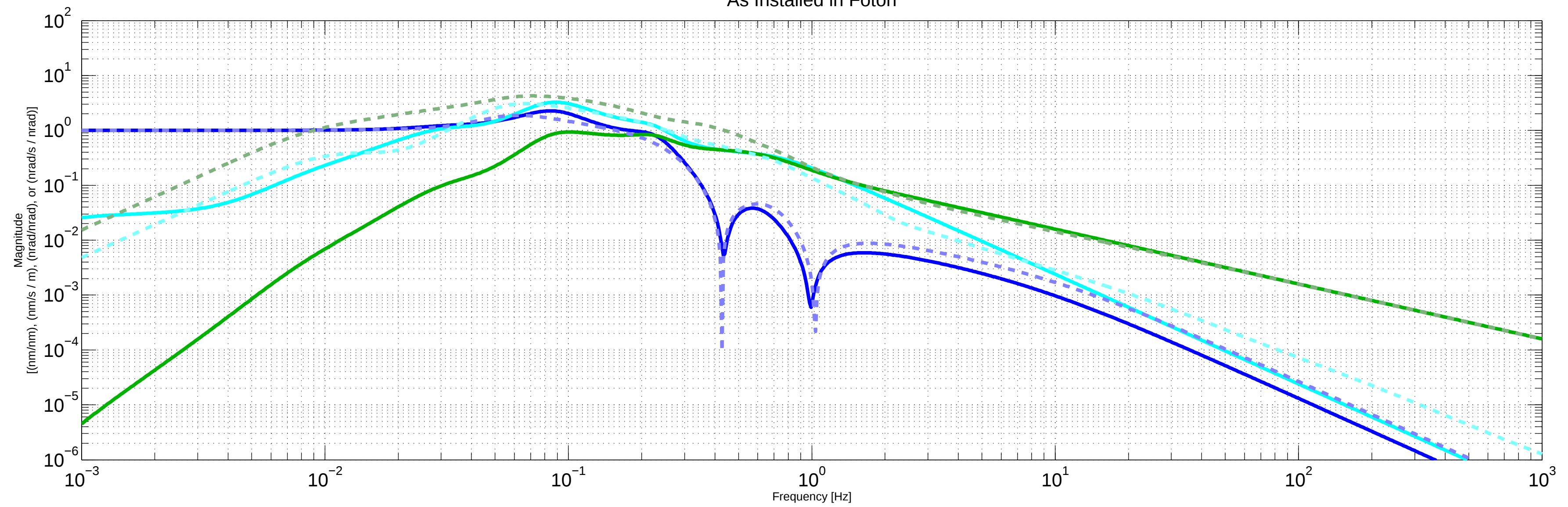
H1ISIETMX ST1 X Quite and rdr Blend Filters As Installed in Foton
