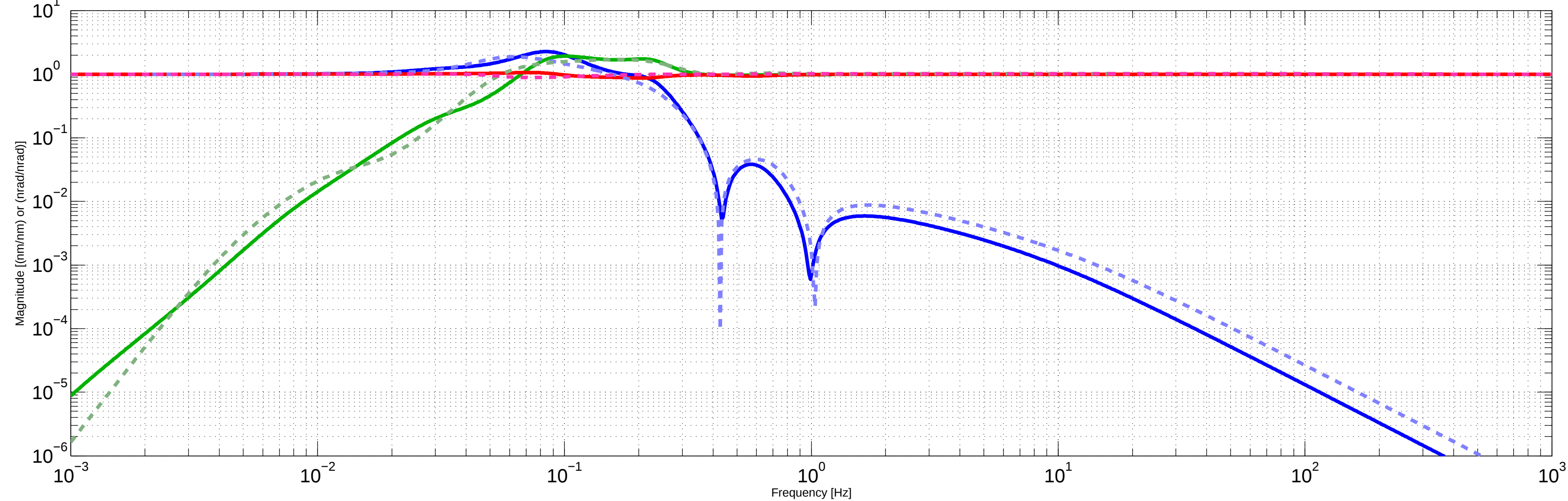
H1ISIETMX ST1 X Quite and rdr Blend Filters Displacement LP vs Inertial HP, As Designed Complementarity
