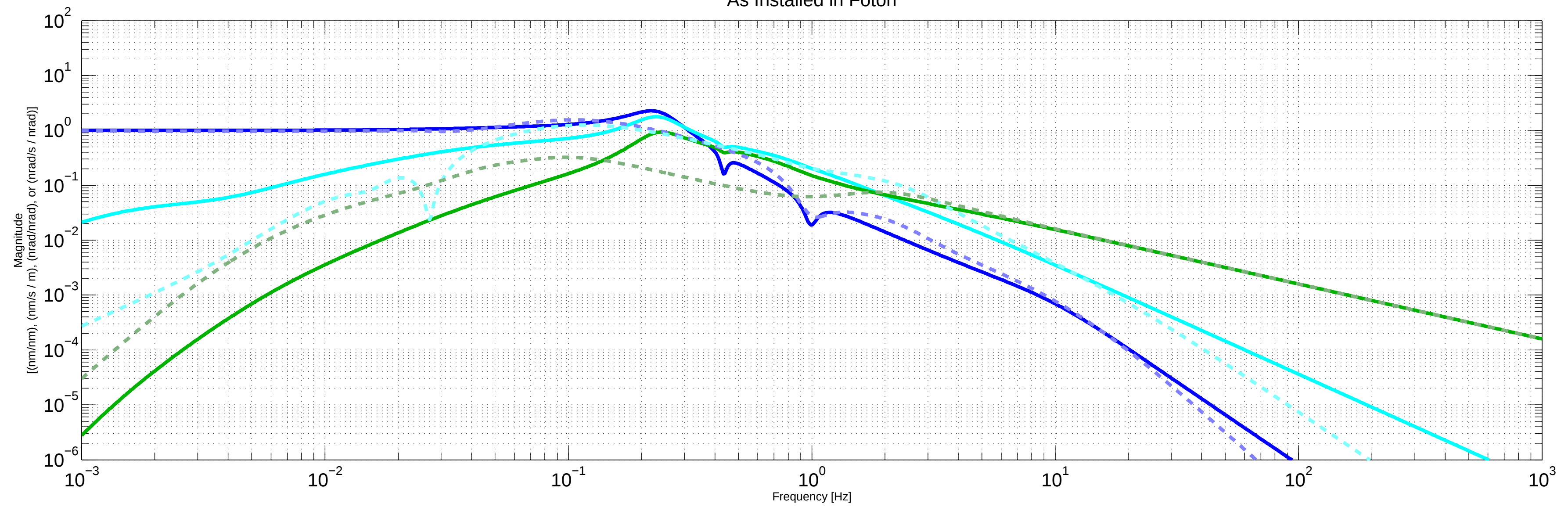
H1ISIETMX ST1 RY Quite and rdr Blend Filters As Installed in Foton
