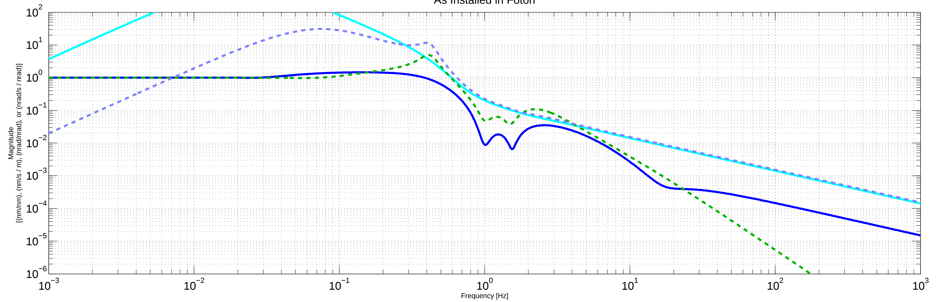
H1ISIHAM2 ST1 X Quite and rdr Blend Filters As Installed in Foton
