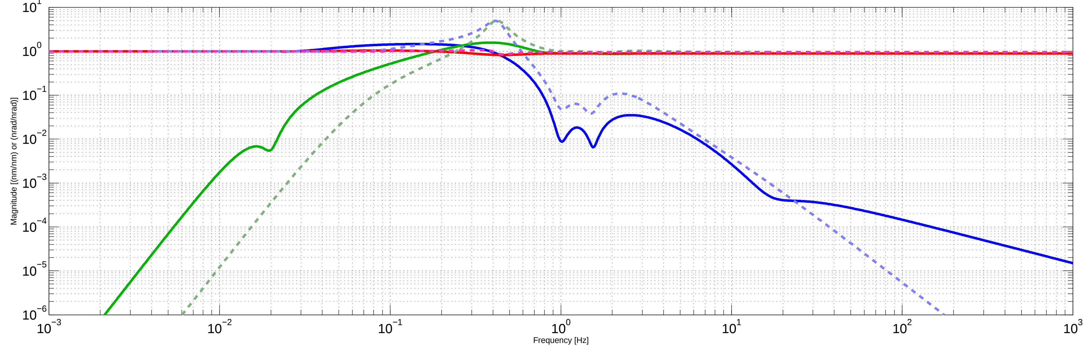
H1ISIHAM2 0128 X and RY Blend Filters Displacement LP vs Inertial HP, As Designed Complementarity
