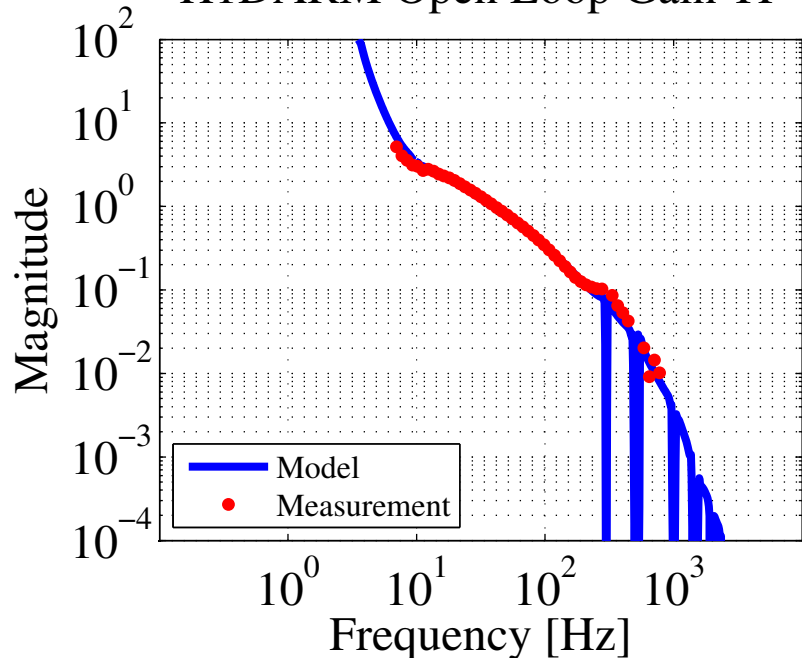
H1DARM Open Loop Gain TF
