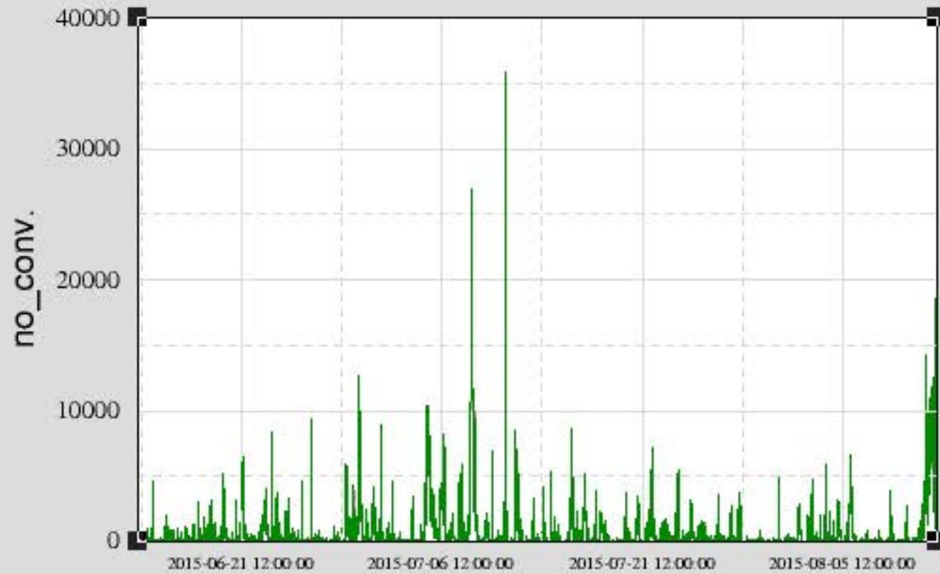
Ch 1: H1:PEM-EY_DUST_VEA1_300NM_PCF
