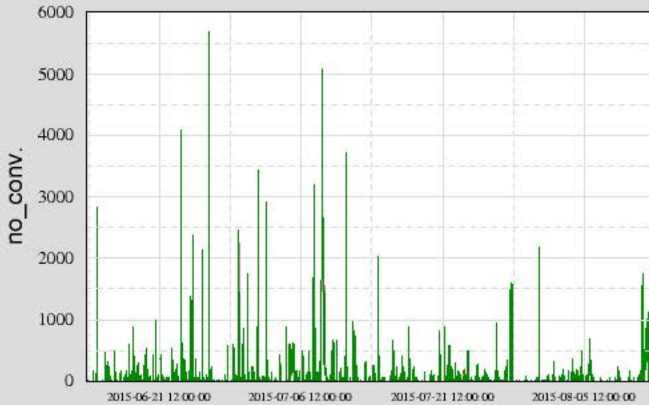
Ch 2: H1:PEM-EY_DUST_VEA1_500NM_PCF
