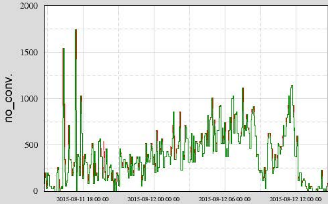
Ch 2: H1:PEM-EY_DUST_VEA1_500NM_PCF
