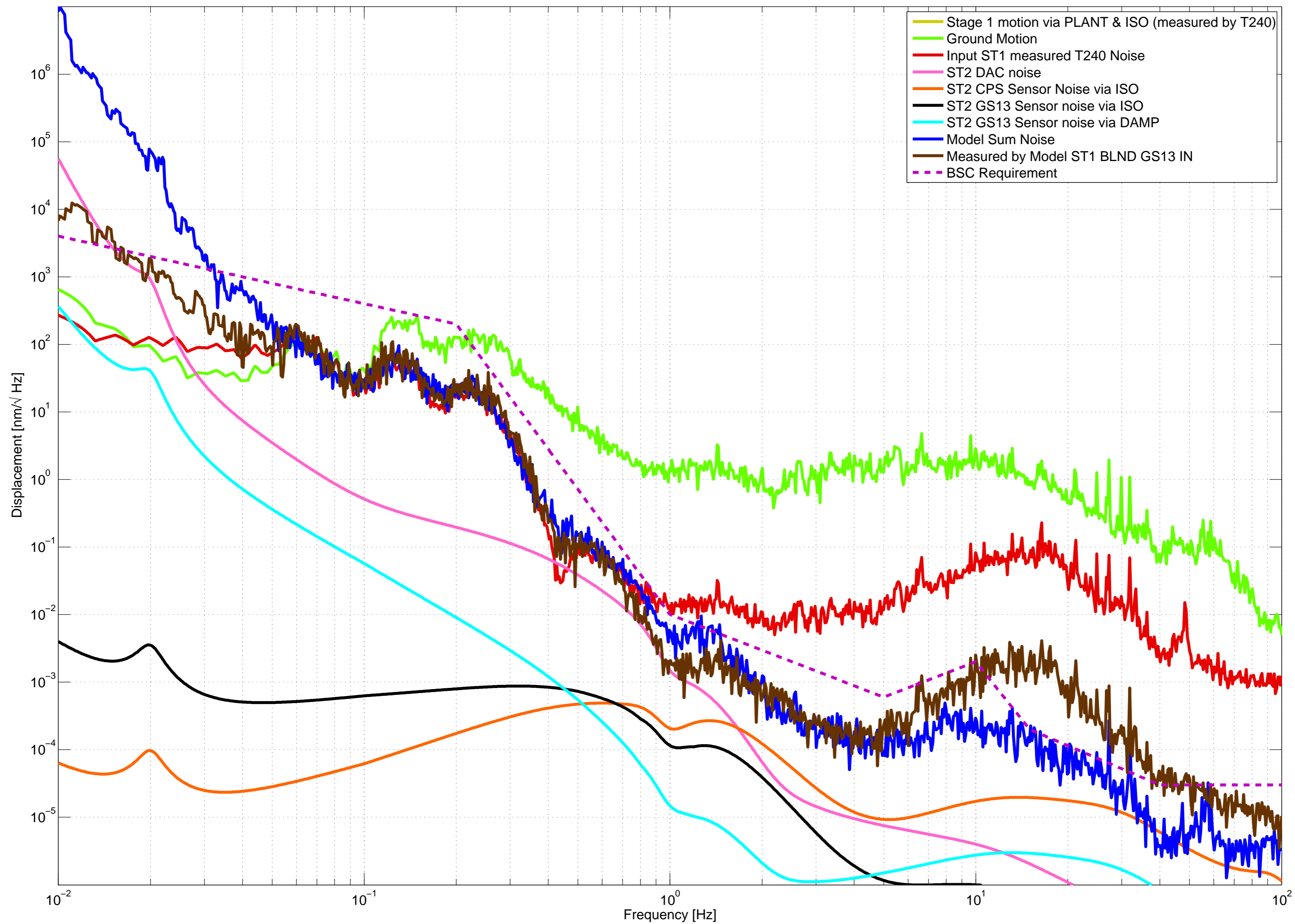
ITMY -ST2 GS13 Z IN1 for GPS 1123326991 generated at 13-Aug-2015 16:22:30
