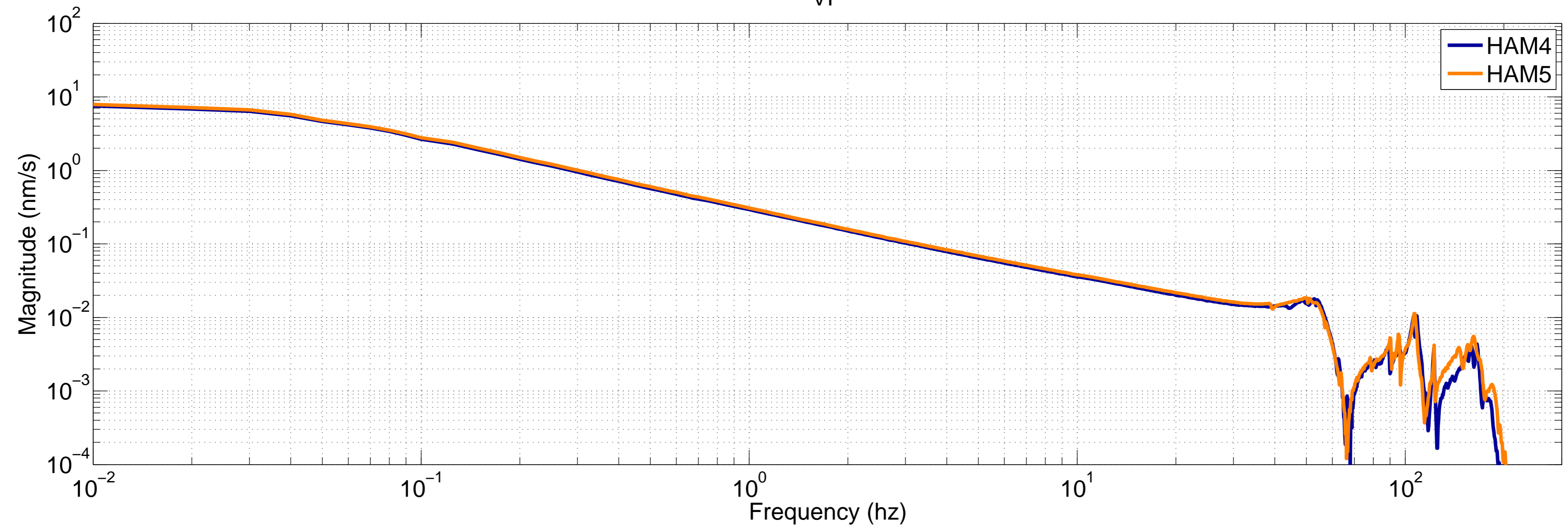
LHO HAM4 & HAM5 HEPI Cart TFs VP
