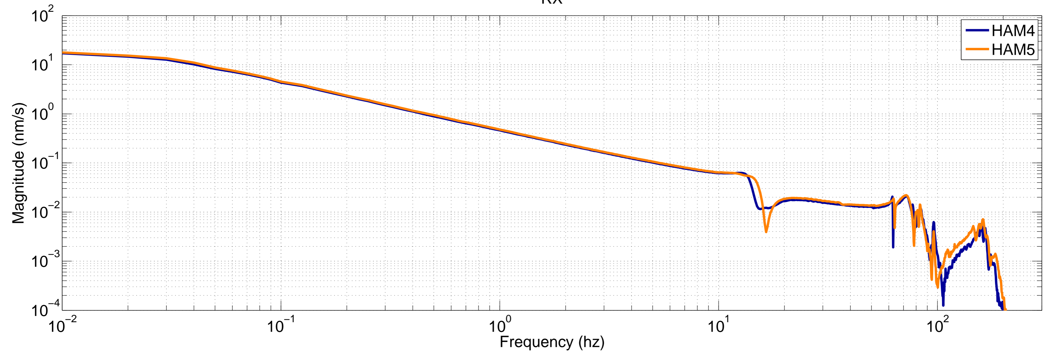
LHO HAM4 & HAM5 HEPI Cart TFs RX
