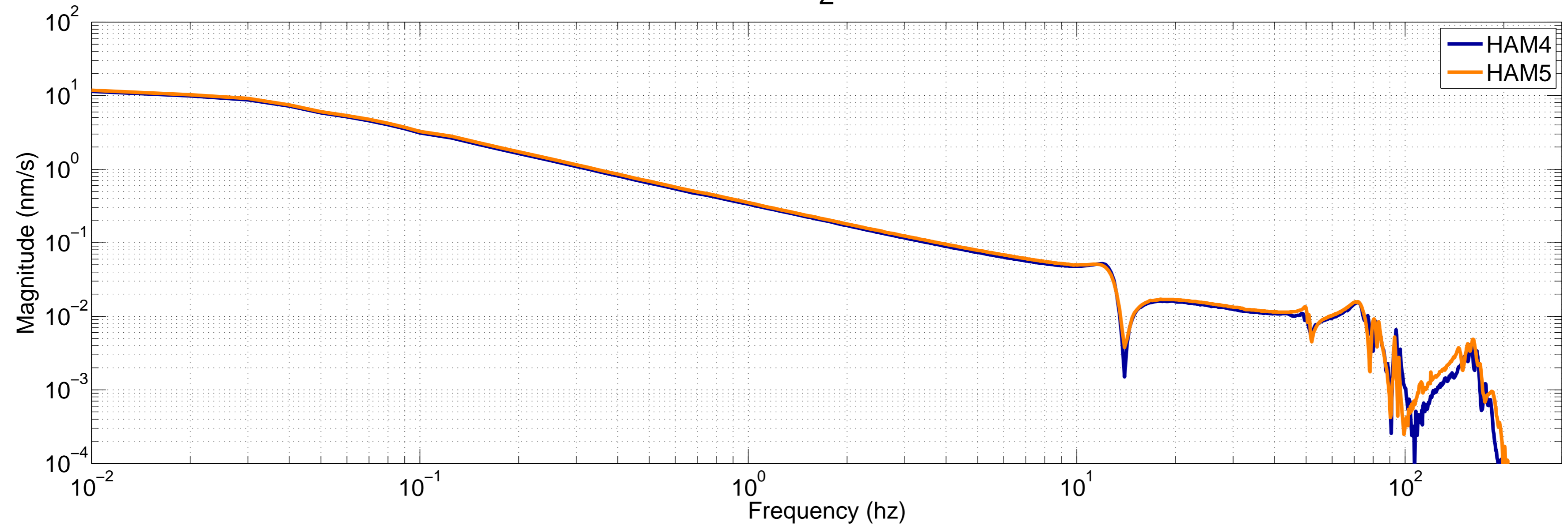
LHO HAM4 & HAM5 HEPI Cart TFs Z
