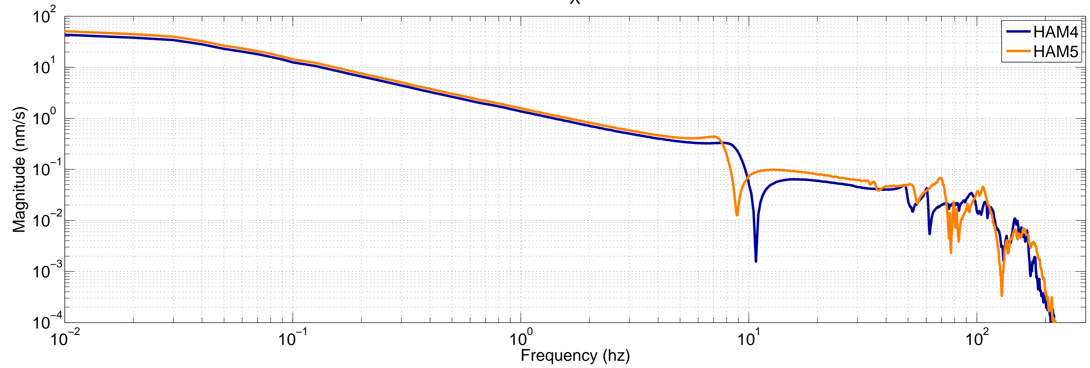
LHO HAM4 & HAM5 HEPI Cart TFs X
