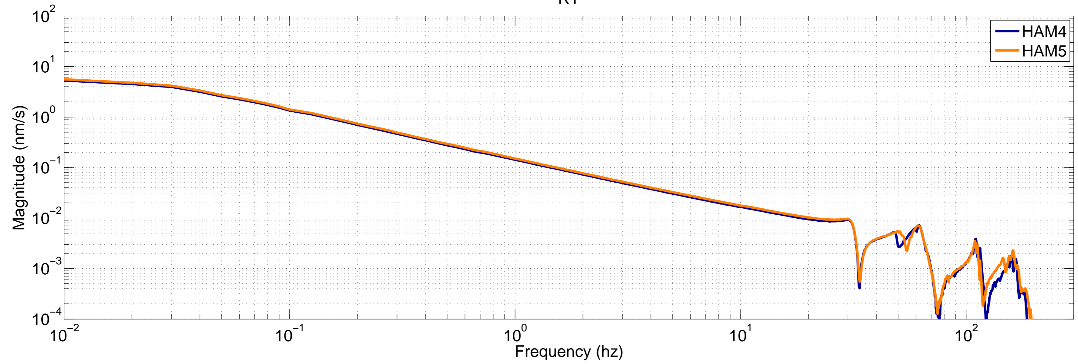
LHO HAM4 & HAM5 HEPI Cart TFs RY
