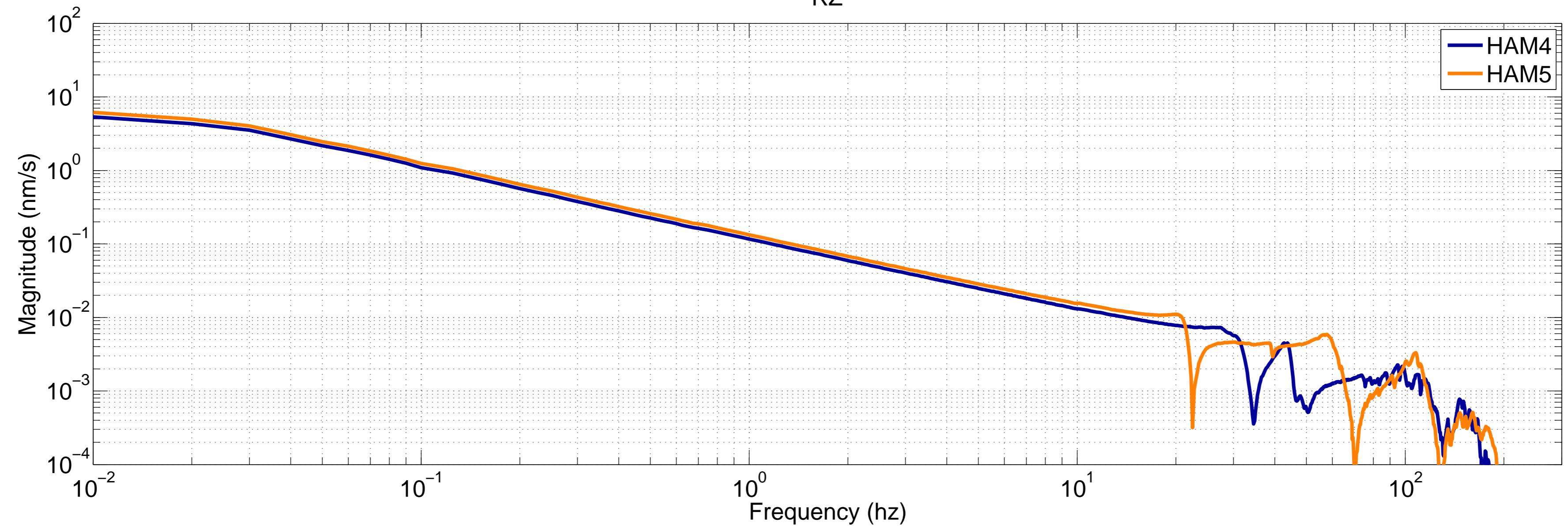
LHO HAM4 & HAM5 HEPI Cart TFs RZ
