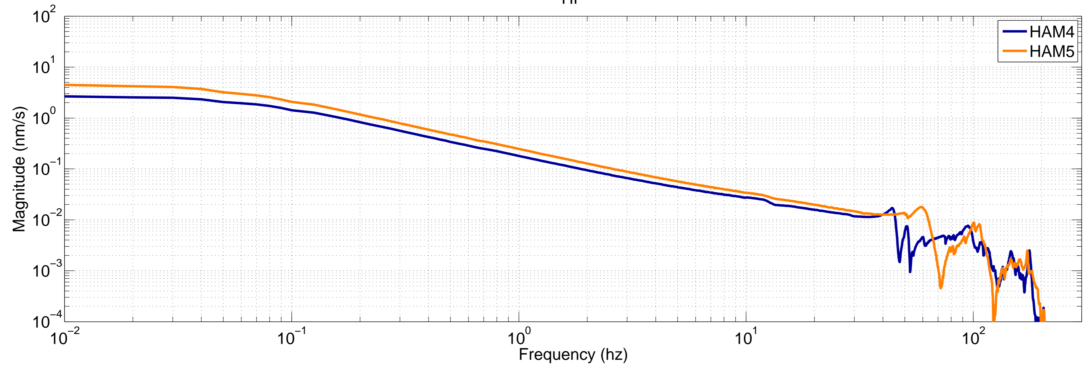
LHO HAM4 & HAM5 HEPI Cart TFs HP
