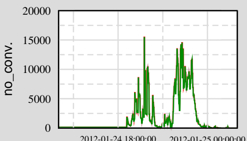
Ch 1: H0:PEM-LVEA_DST1_5
