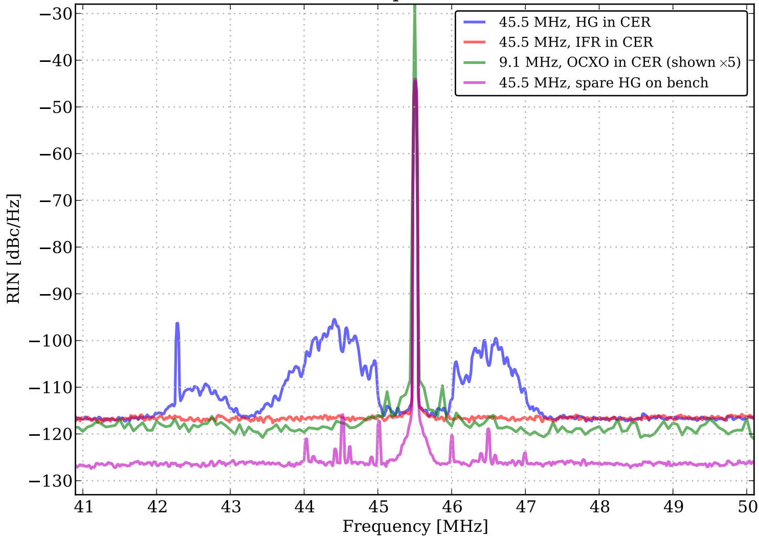
RF oscillator spectra, 2015-08-27
