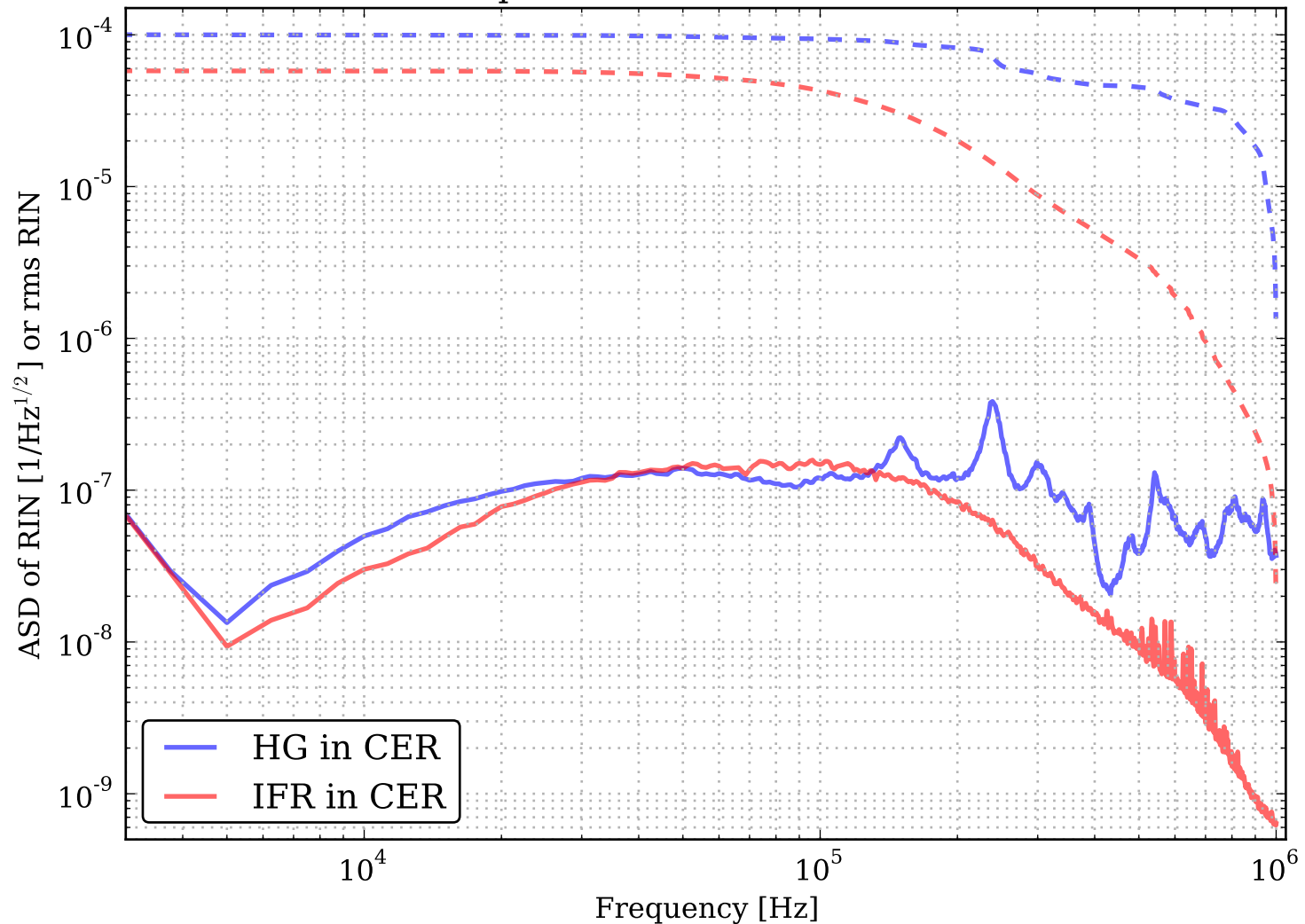
Out-of-loop 45.5 MHz RIN after EOM driver
