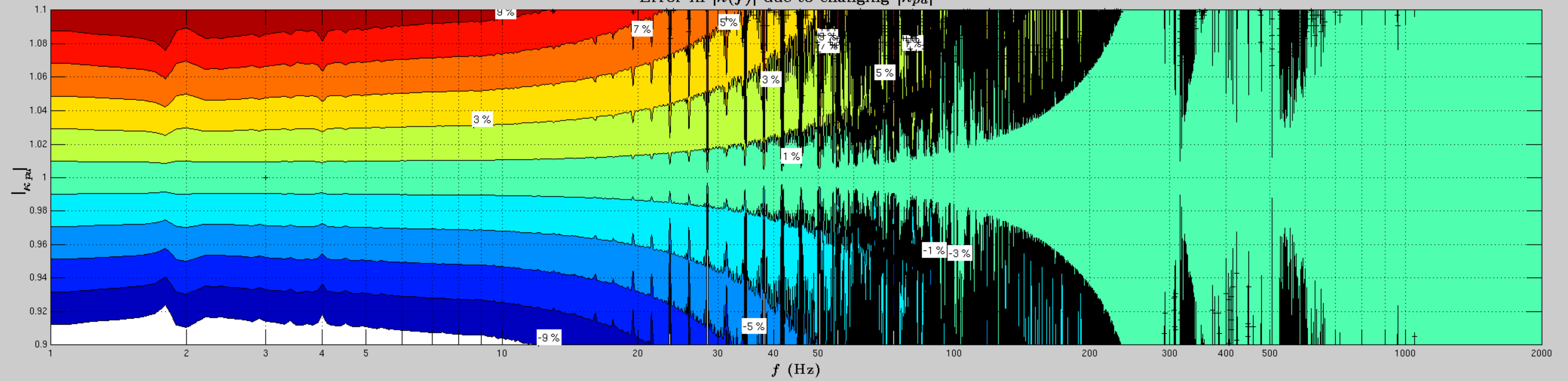
Error in |h(f)| due to changing |\kappa_{pu}|
