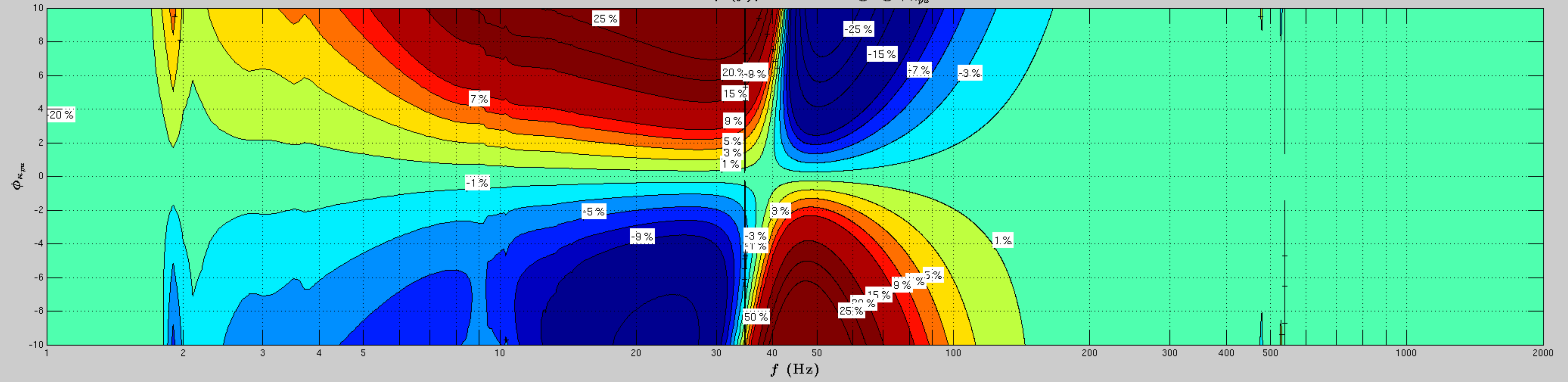
Error in |h(f)| due to changing \phi_{\kappa_{\eta u}}
