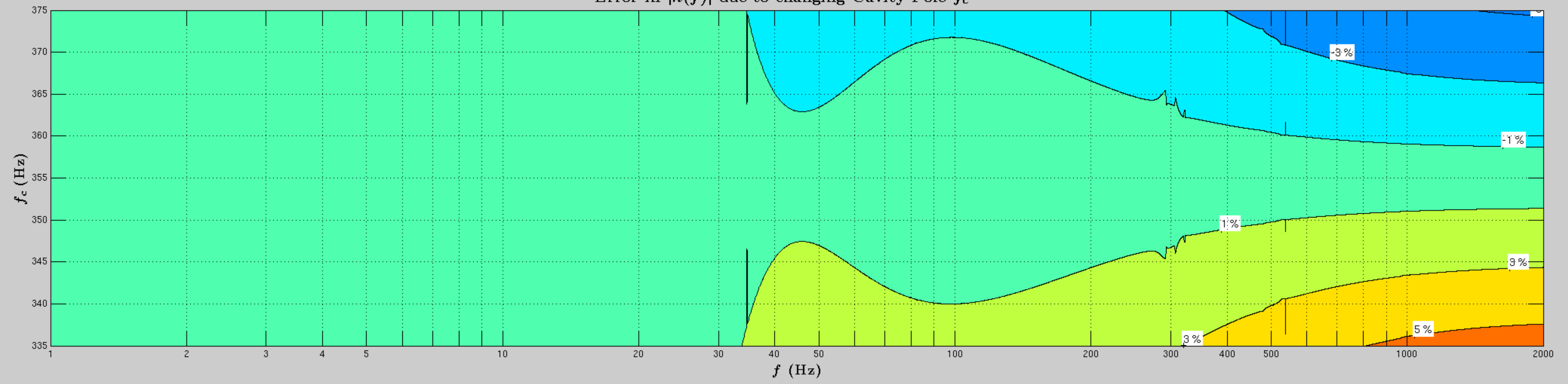
Error in |h(f)| due to changing Cavity Pole f_c
