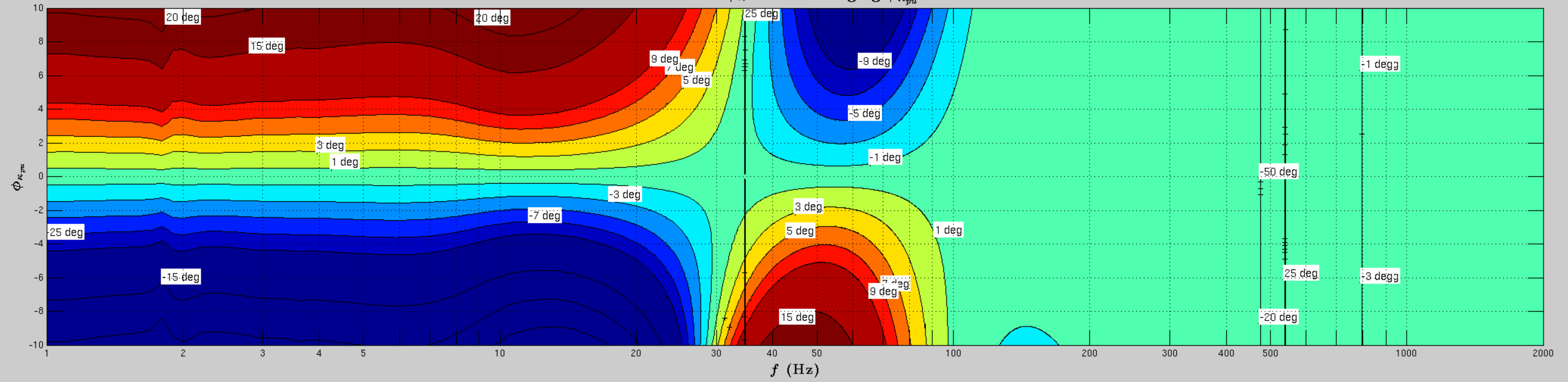
Error in \phi_h due to changing \phi_{\kappa_{pv}}
