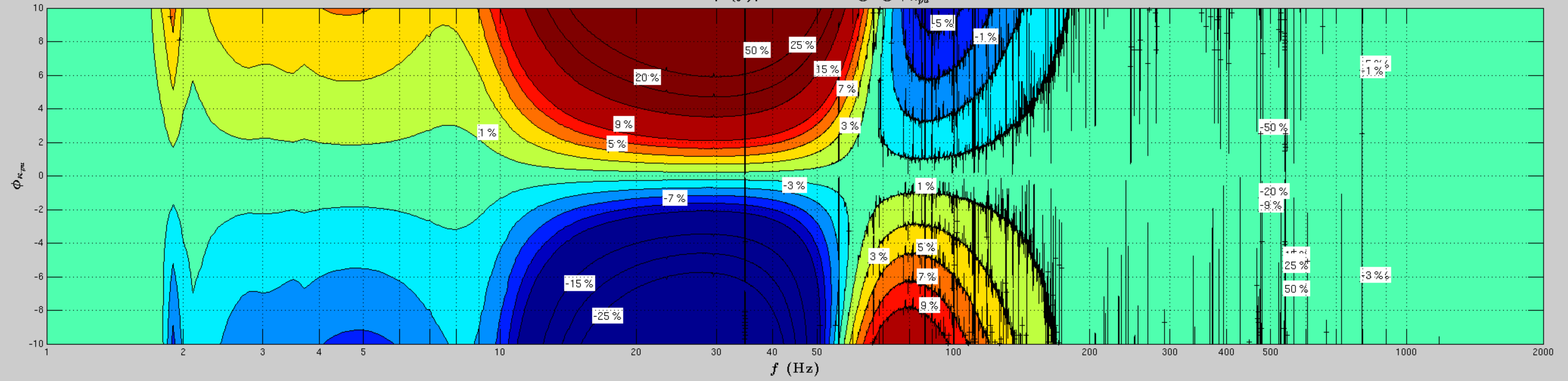
Error in |h(f)| due to changing \phi_{\kappa_{pv}}
