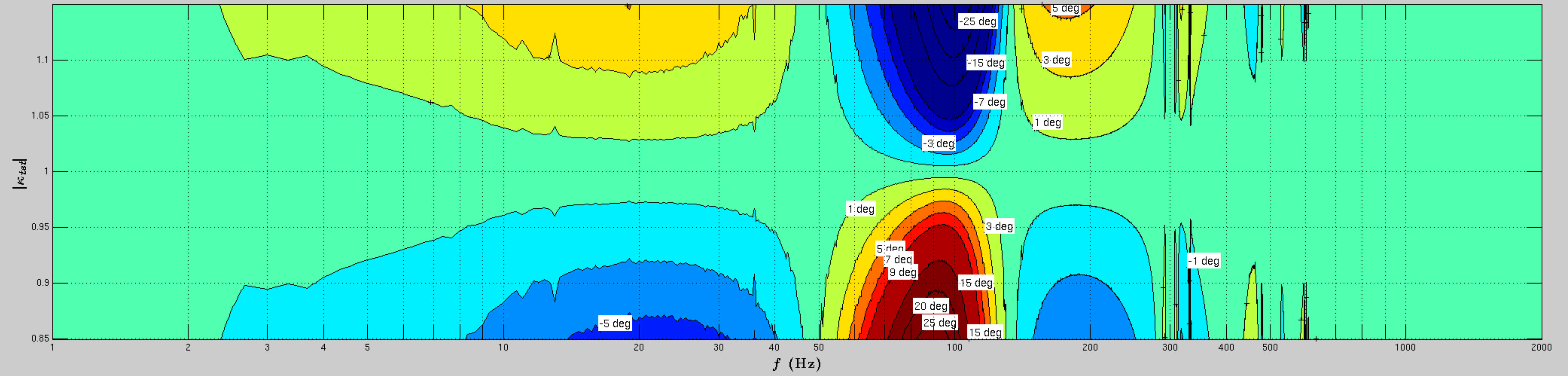
Error in \phi_h due to changing |\kappa_{tst}|
