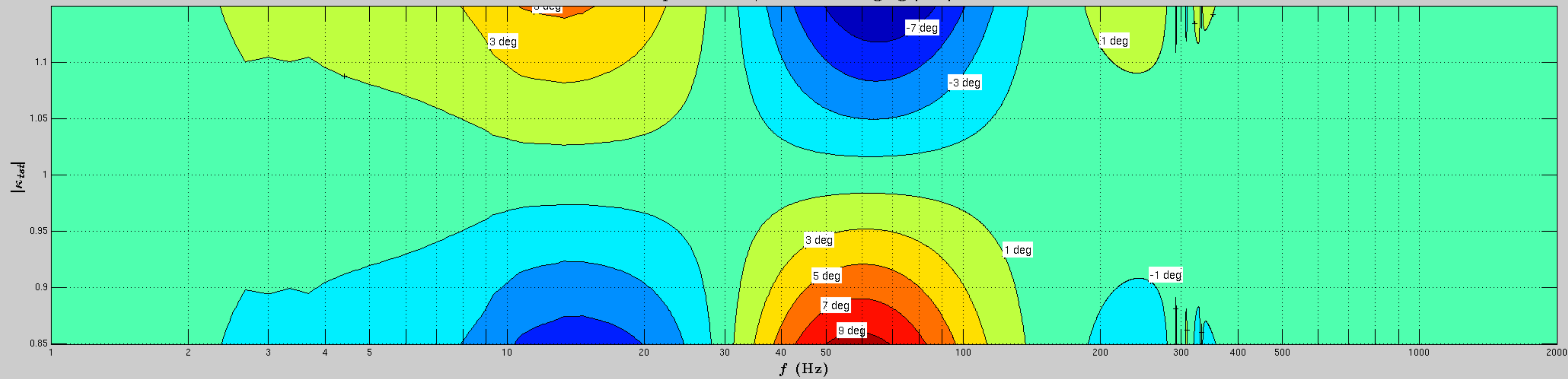
Tmp Error in \phi_h due to changing |\kappa_{tst}|
