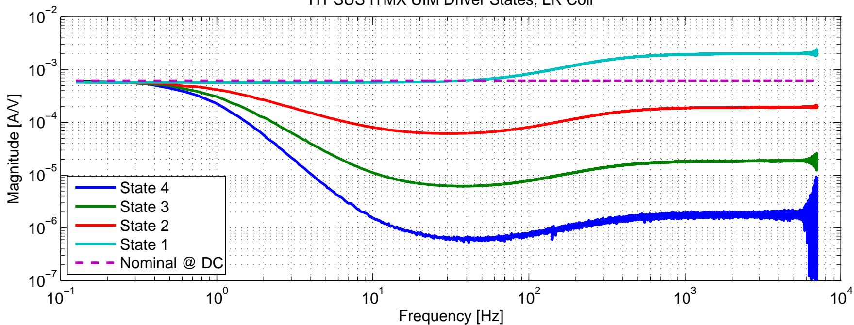
H1 SUS ITMX UIM Driver States, LR Coil
