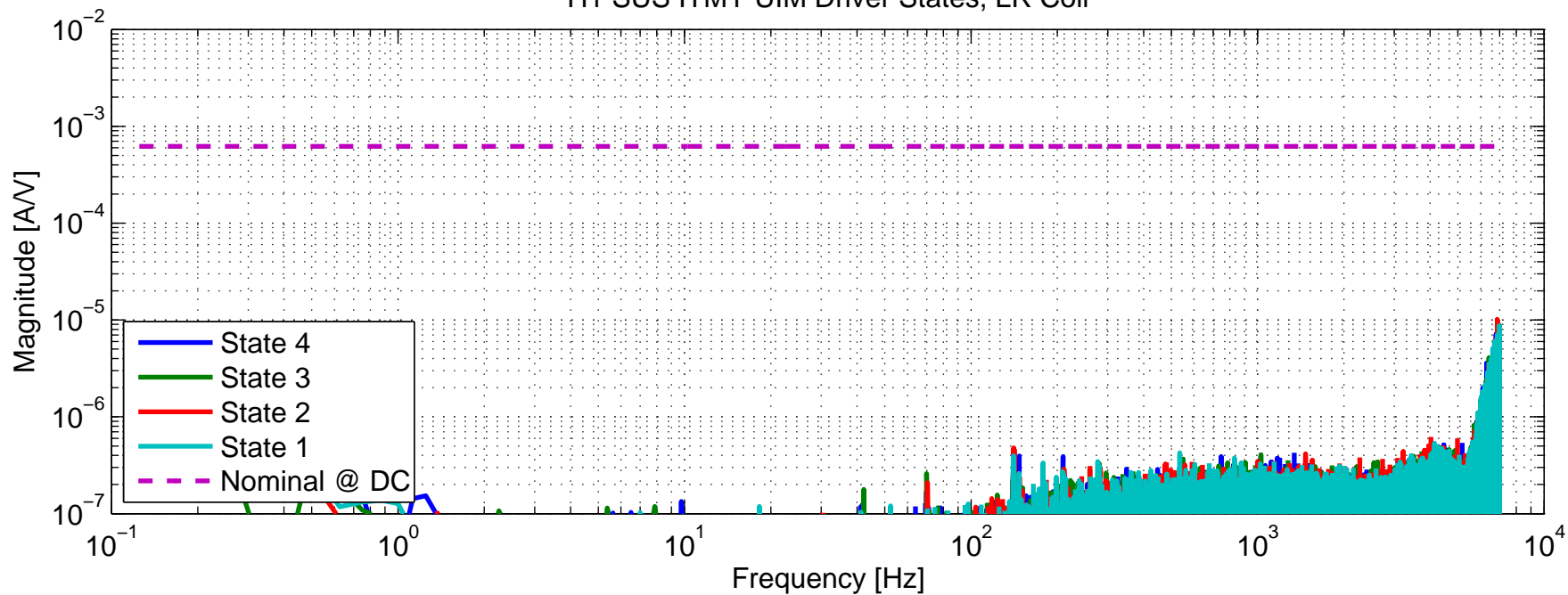
H1 SUS ITMY UIM Driver States, LR Coil
