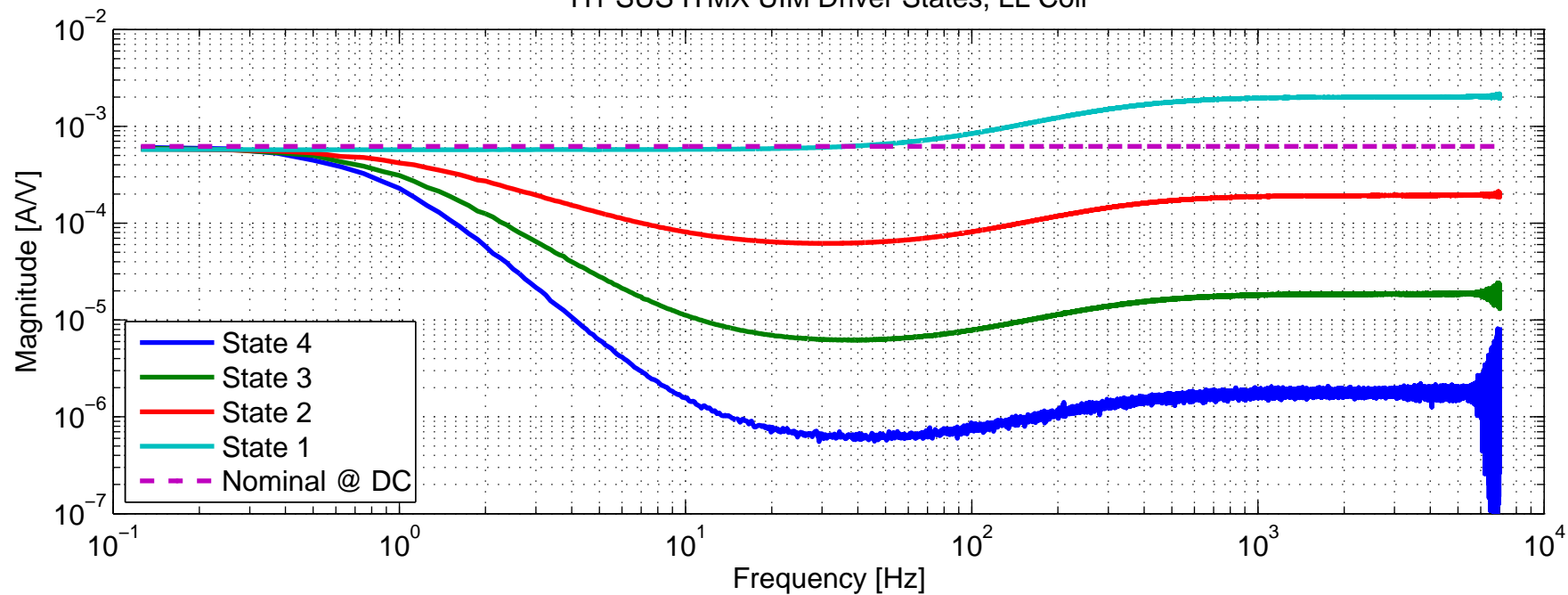
H1 SUS ITMX UIM Driver States, LL Coil
