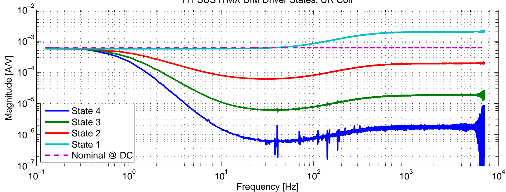
H1 SUS ITMX UIM Driver States, UR Coil
