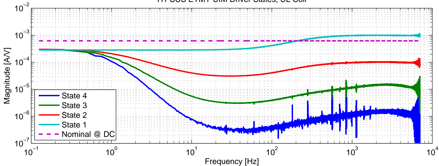
H1 SUS ETMY UIM Driver States, UL Coil
