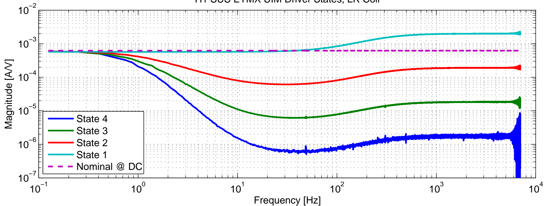
H1 SUS ETMX UIM Driver States, LR Coil
