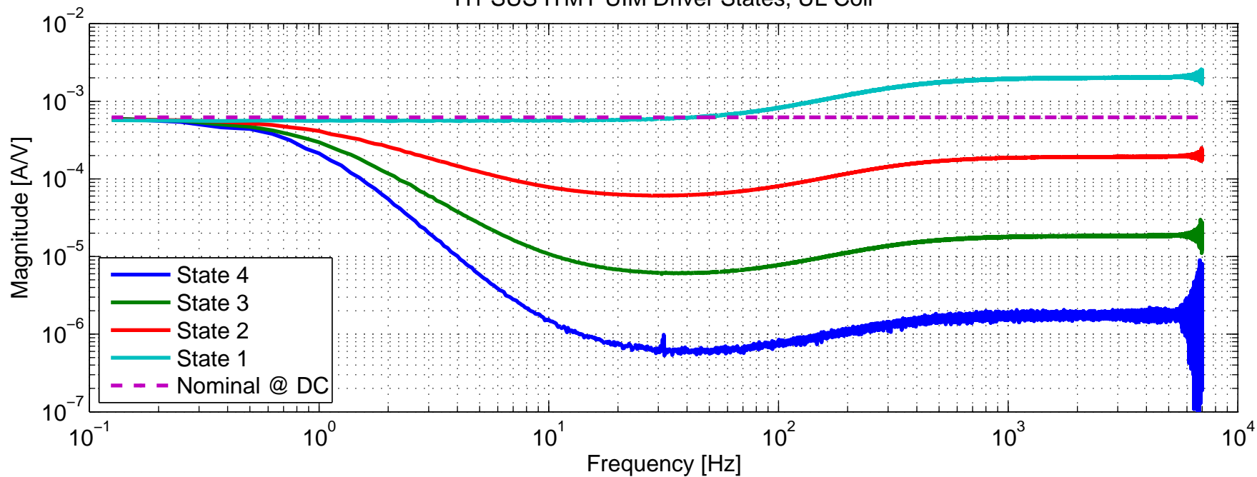
H1 SUS ITMY UIM Driver States, UL Coil
