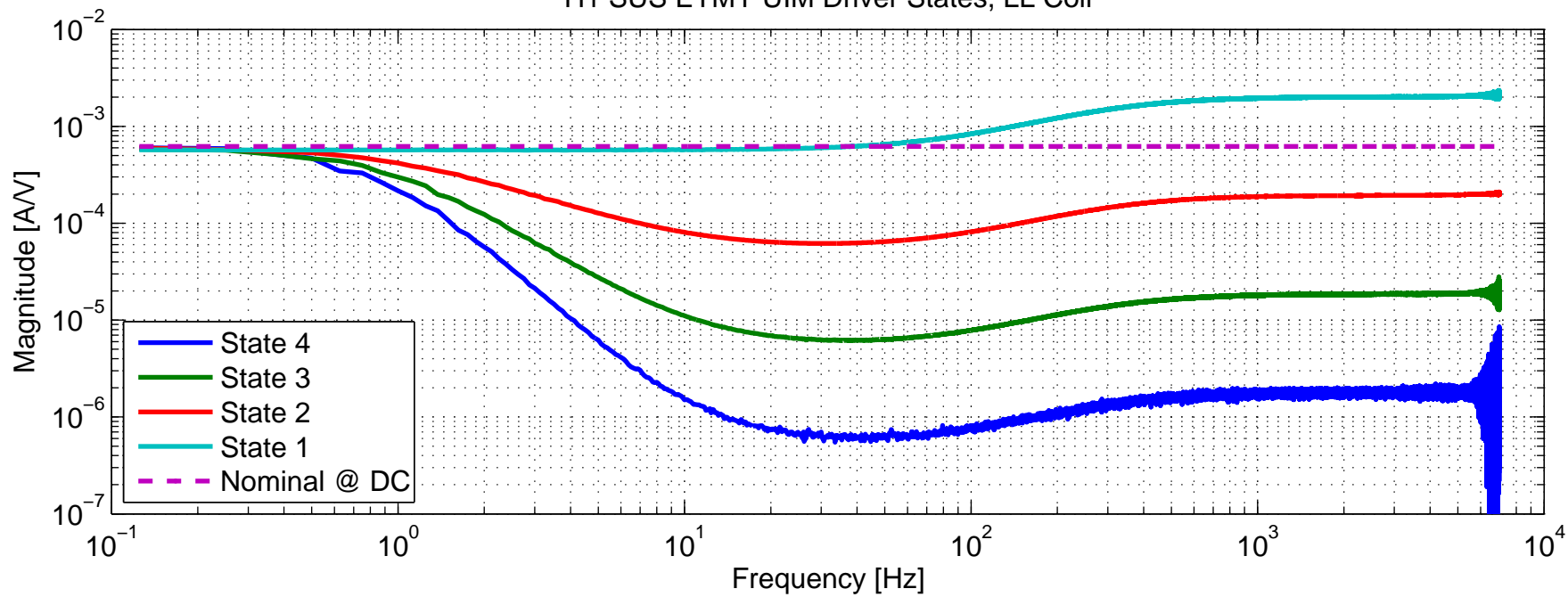
H1 SUS ETMY UIM Driver States, LL Coil
