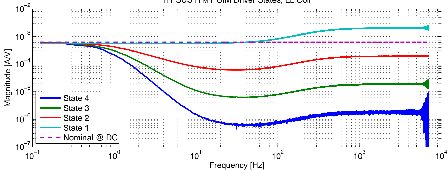
H1 SUS ITMY UIM Driver States, LL Coil
