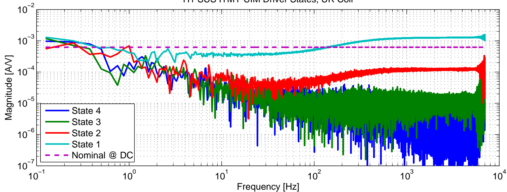
H1 SUS ITMY UIM Driver States, UR Coil
