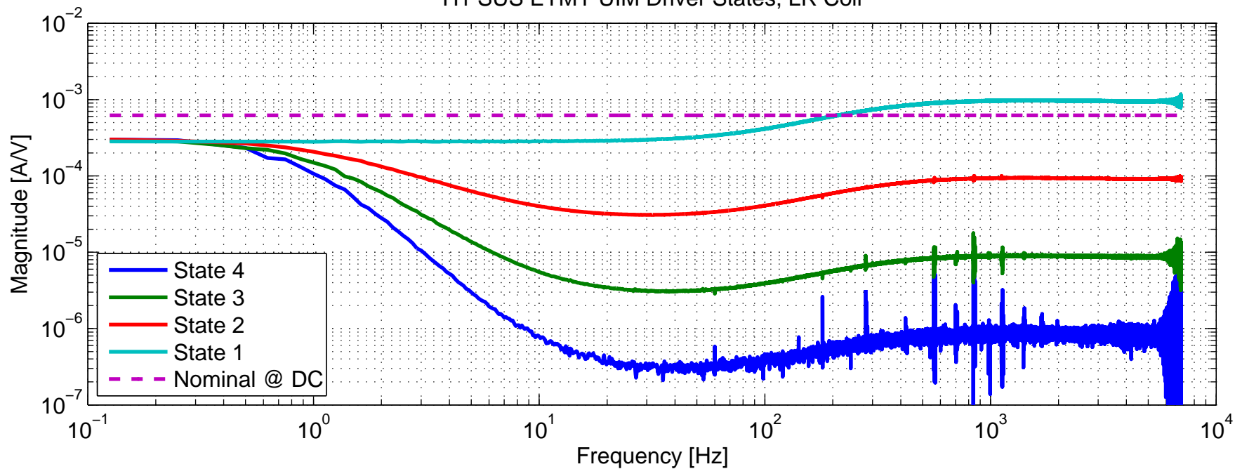
H1 SUS ETMY UIM Driver States, LR Coil
