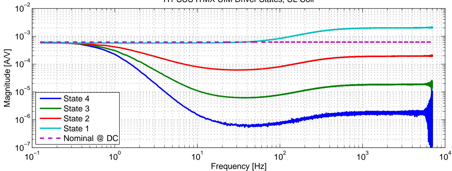
H1 SUS ITMX UIM Driver States, UL Coil
