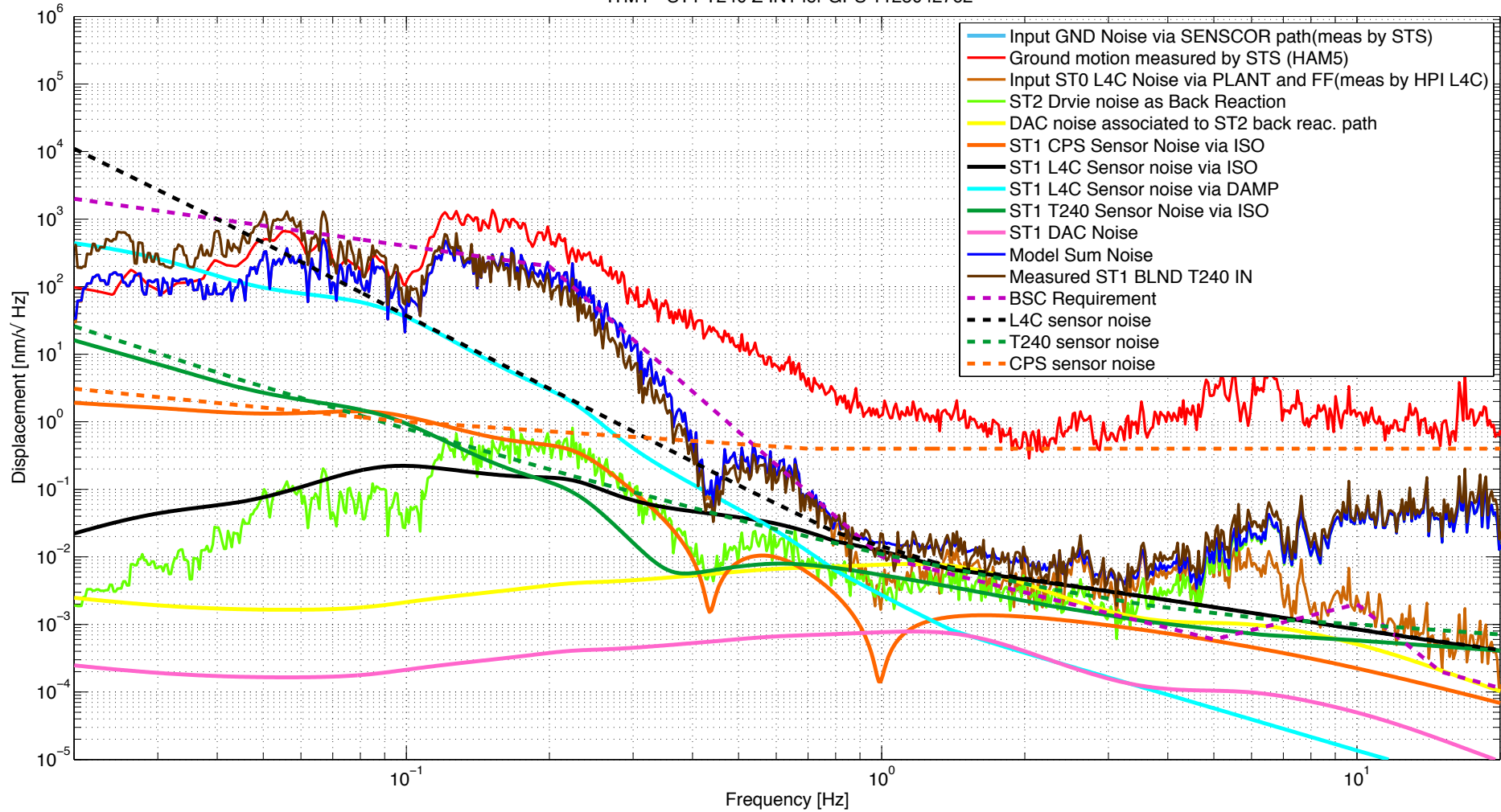
ITMY -ST1 T240 Z IN1 for GPS 1125042762
