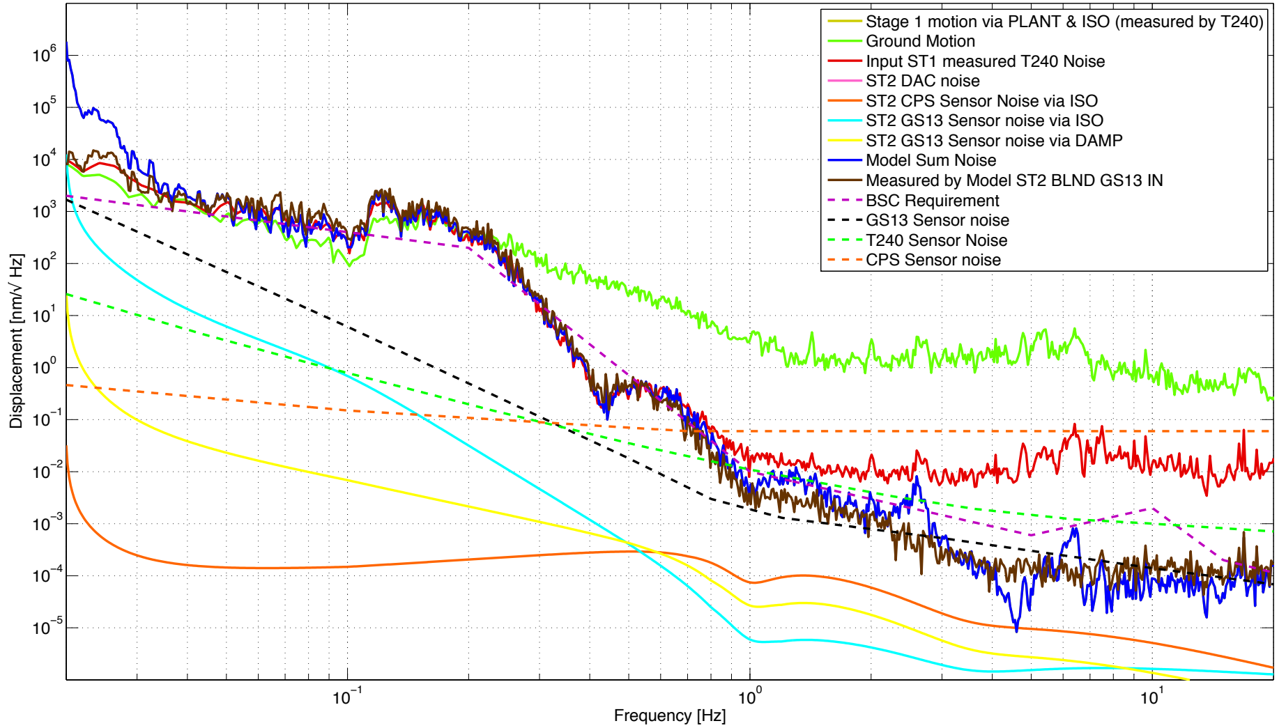
ITMY -ST2 GS13 X IN1 for GPS 1125042762
