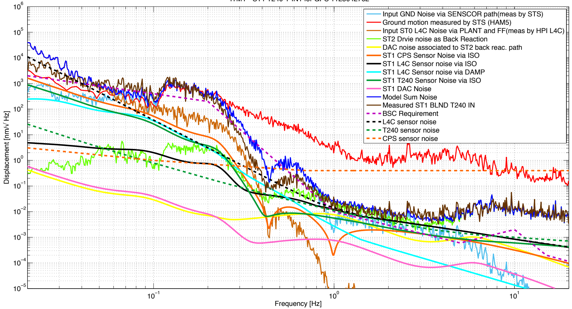
ITMY -ST1 T240 Y IN1 for GPS 1125042762
