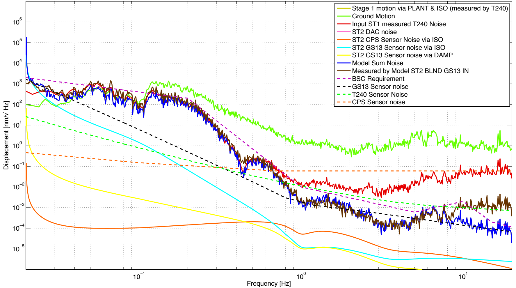
ITMY -ST2 GS13 Z IN1 for GPS 1125042762
