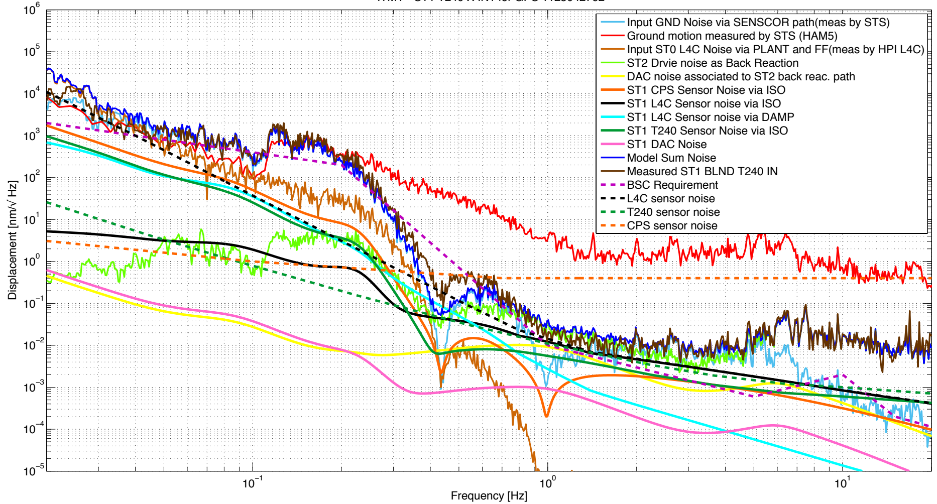
ITMY -ST1 T240 X IN1 for GPS 1125042762
