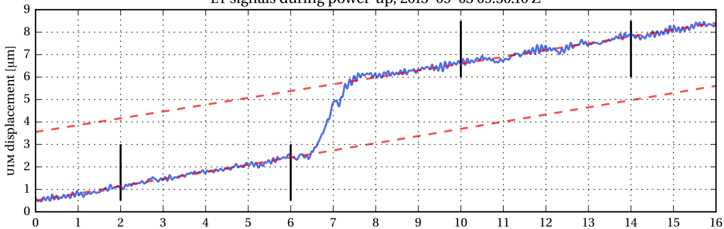
EY signals during power-up, 2015-09-03 09:50:10 Z
