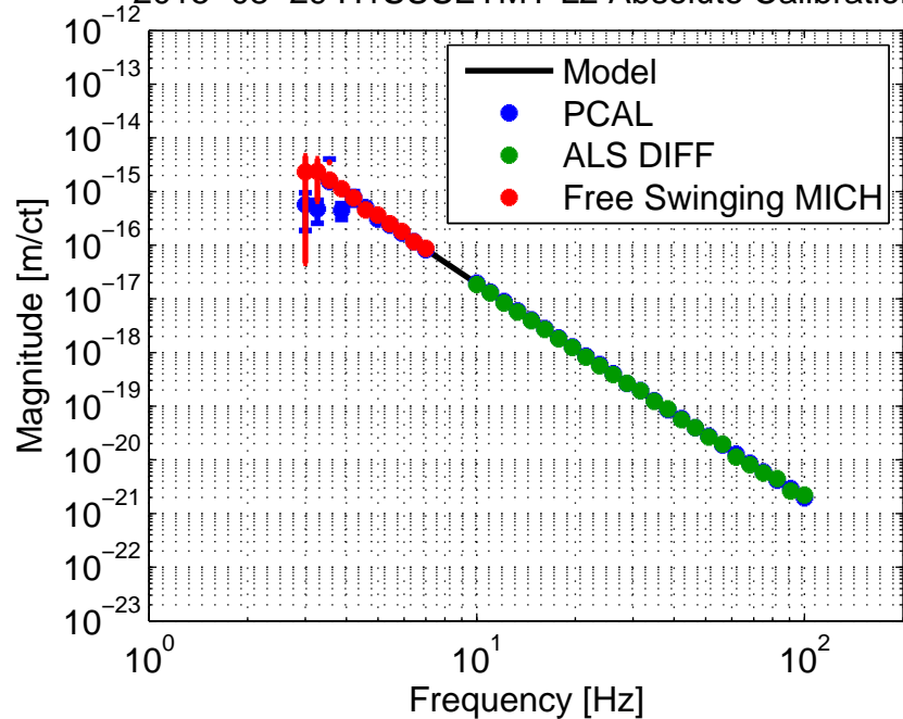
2015-08-29 H1SUSEMY L2 Absolute Calibration
