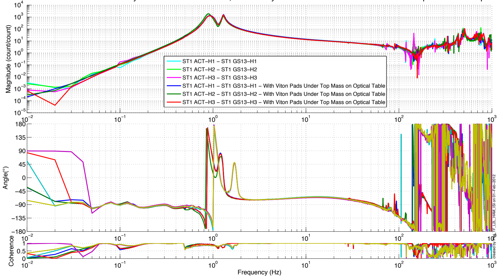
HAM-ISI – LHO – Unit #1 – February 1st 2012 – On test stand, In air – Payload: Masses – Viton Pads Under the Top Mass of the Optical Table
