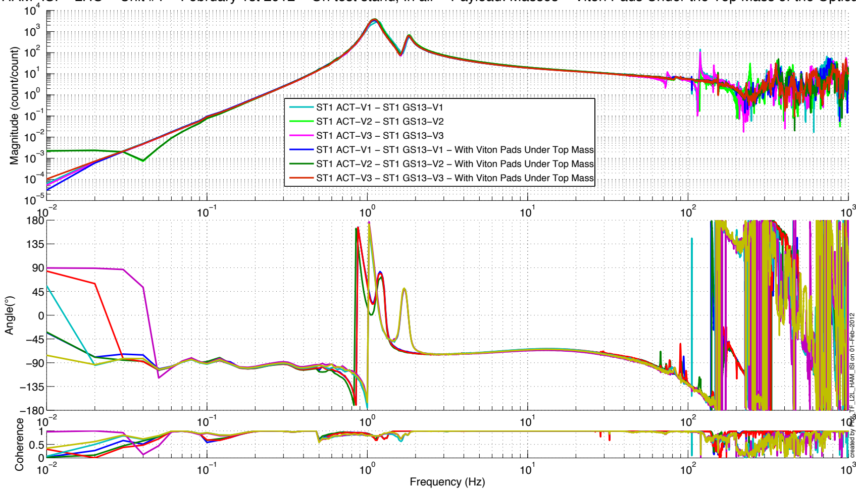
HAM-ISI - LHO - Unit #1 - February 1st 2012 - On test stand, In air - Payload: Masses - Viton Pads Under the Top Mass of the Optical Table
