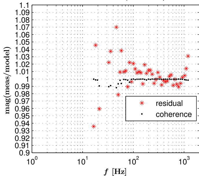
Sensing Residual (meas / model)
