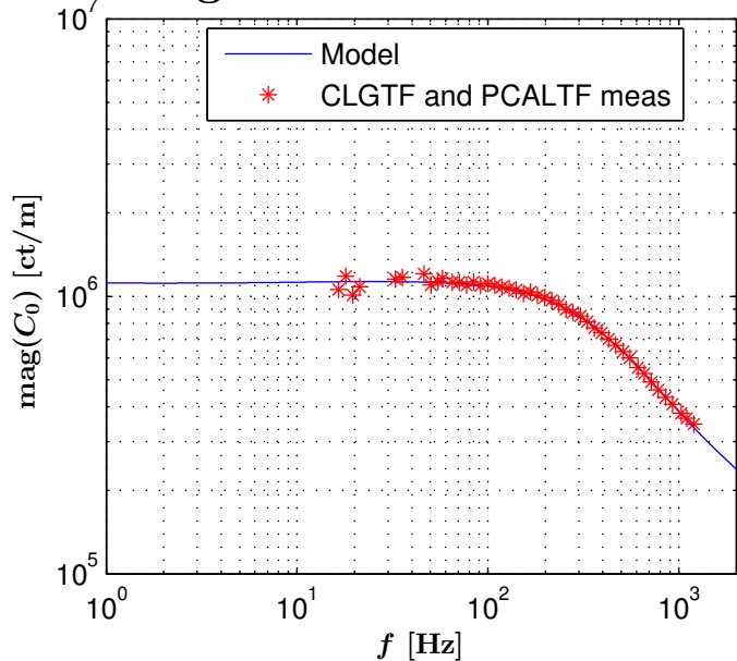
Sensing function vs measurement
