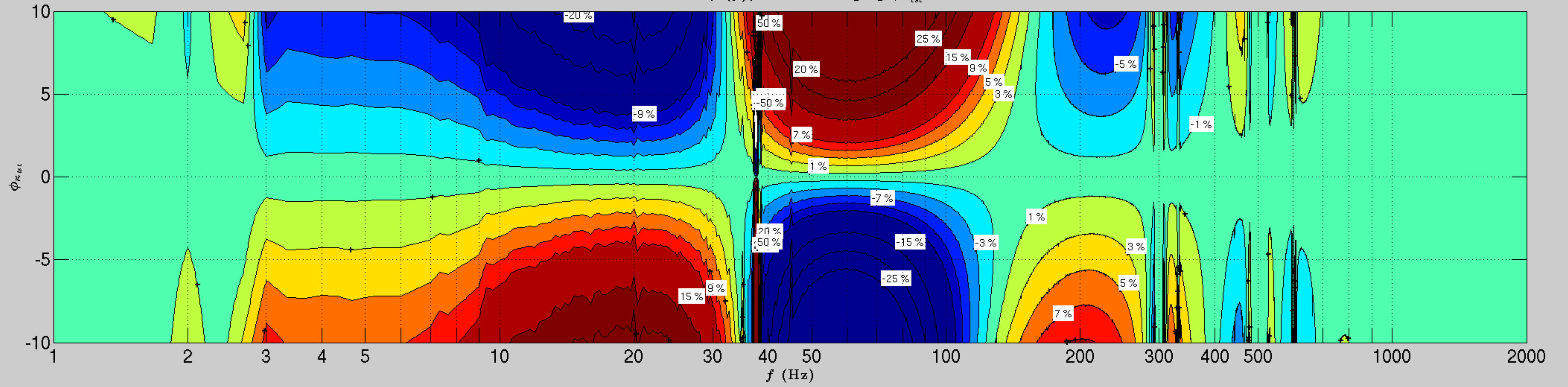
Error in |h(f)| due to changing \phi_{\kappa_{tot}}
