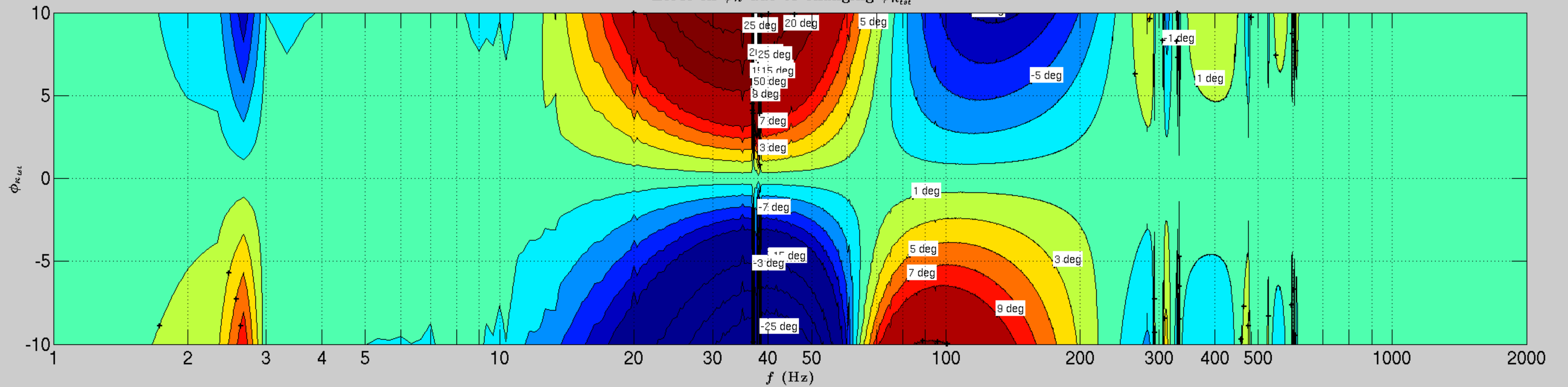
Error in \phi_h due to changing \phi_{\kappa_{tot}}
