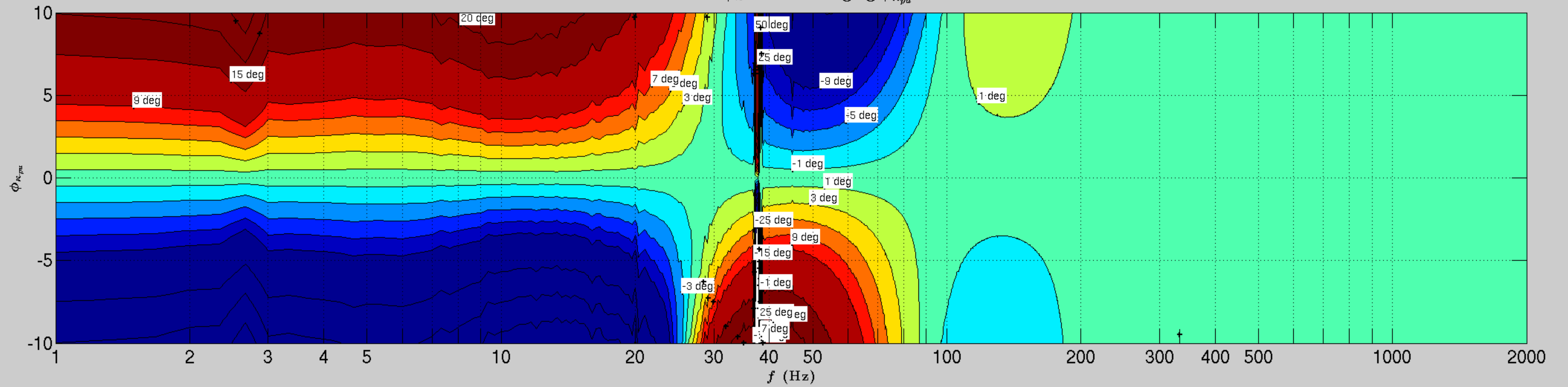
Error in \phi_h due to changing \phi_{\kappa_{pu}}
