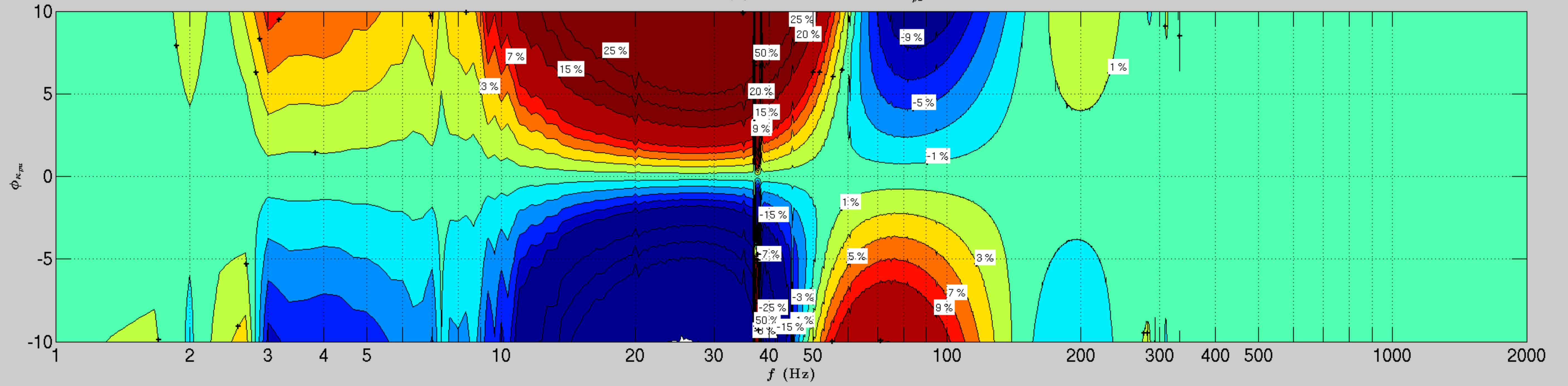
Error in |h(f)| due to changing \phi_{\kappa_{pu}}
