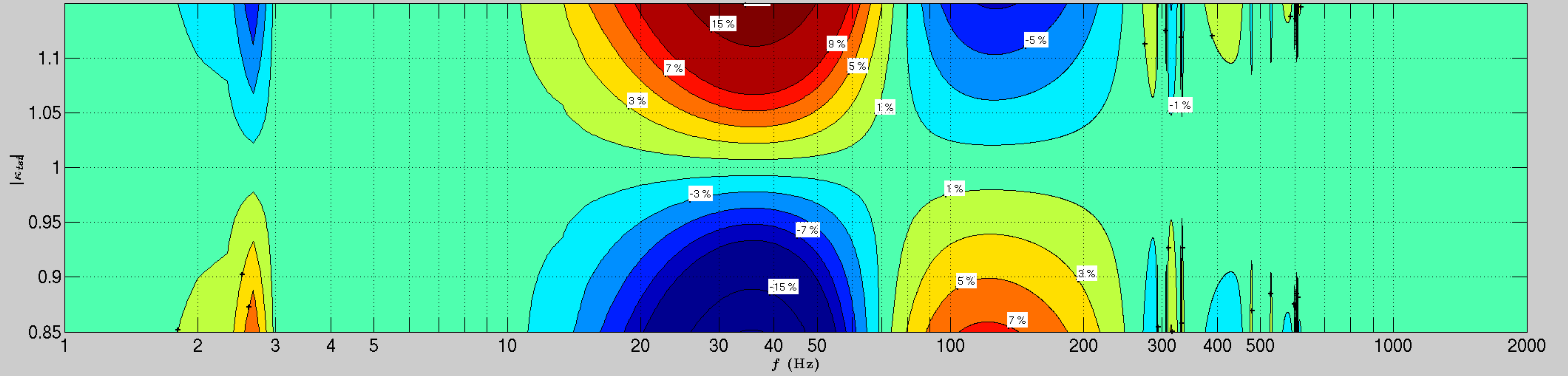
Tmp Error in |h(f)| due to changing |\kappa_{tst}|
