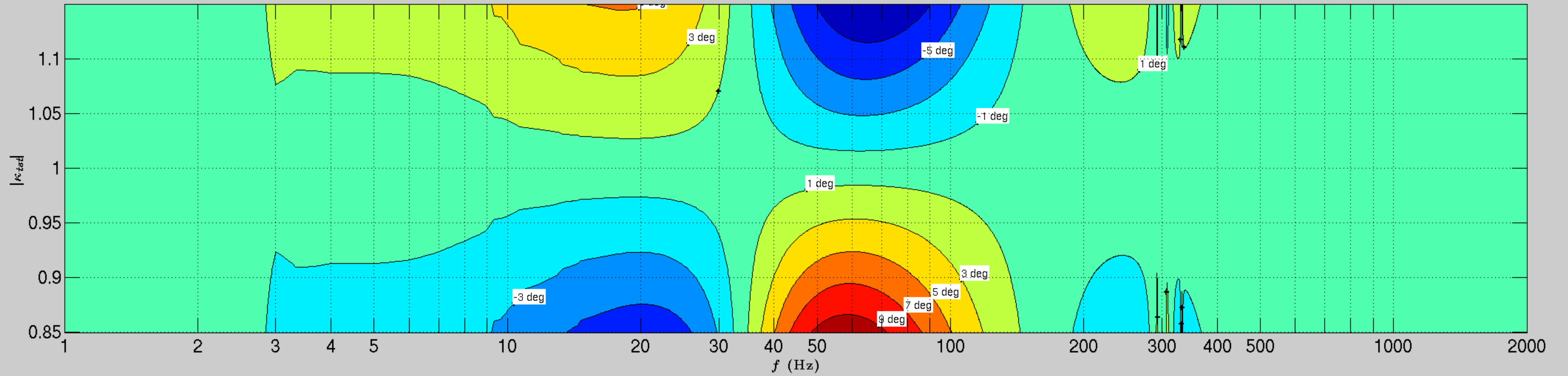
Tmp Error in \phi_h due to changing |\kappa_{tst}|
